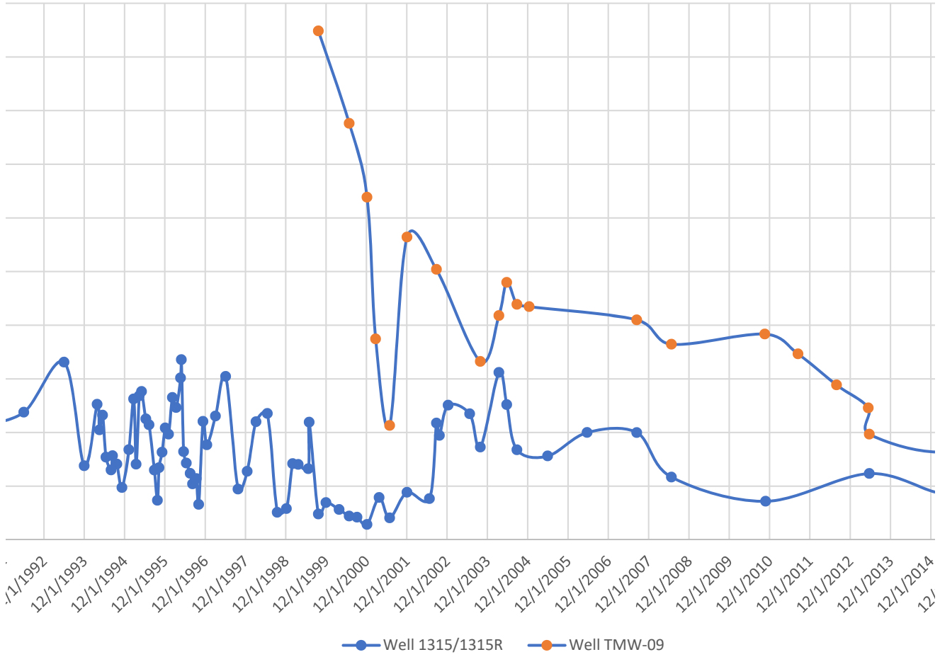
Uranium Concentration (pCi/L to 2016, then ug/L for Well 1315R)
