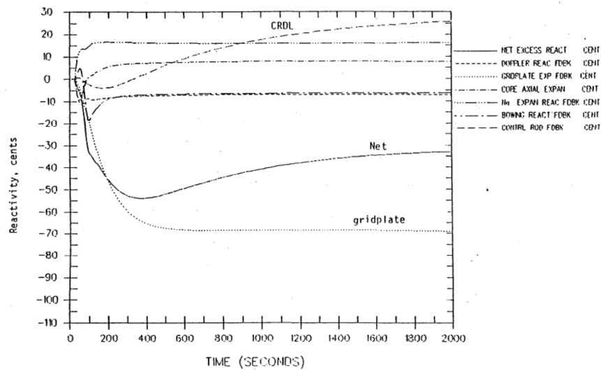
Figure 3.5.N-2. Reactivity
