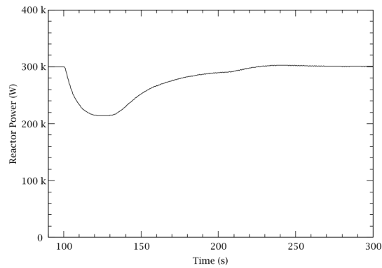
Figure 3.3.N-2. Core Power
