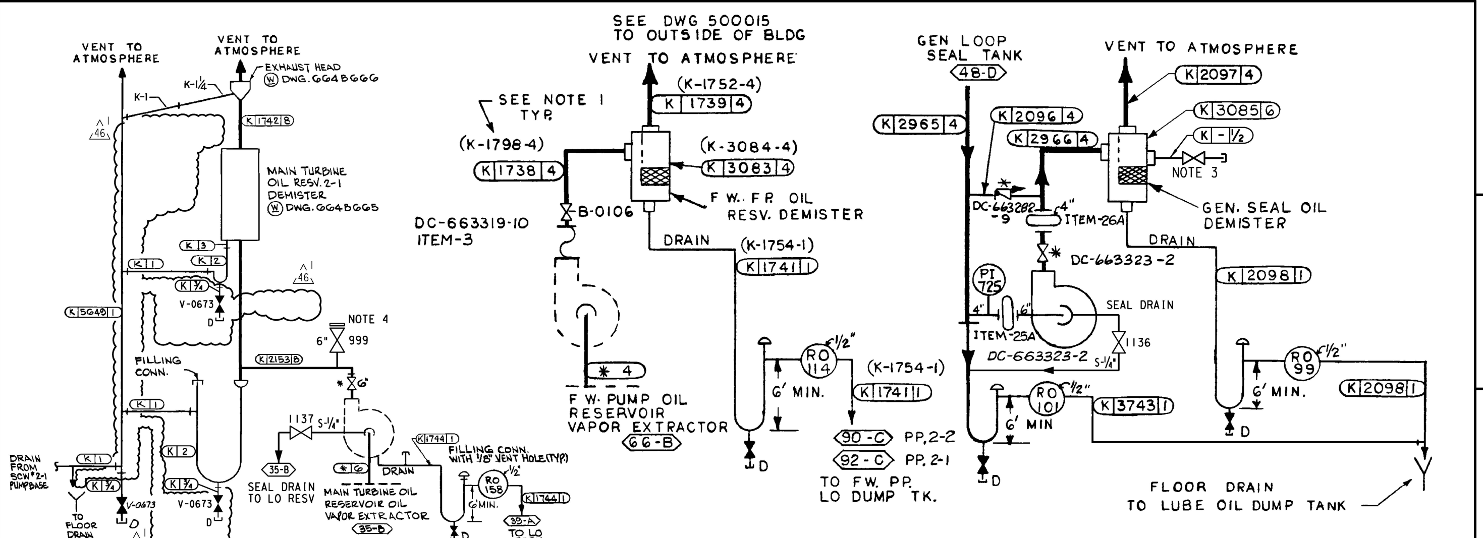
FEEDWATER PUMP OIL RESERVOIR 2-2 VAPOR EXTRACTOR & DEMISTER SYSTEM
