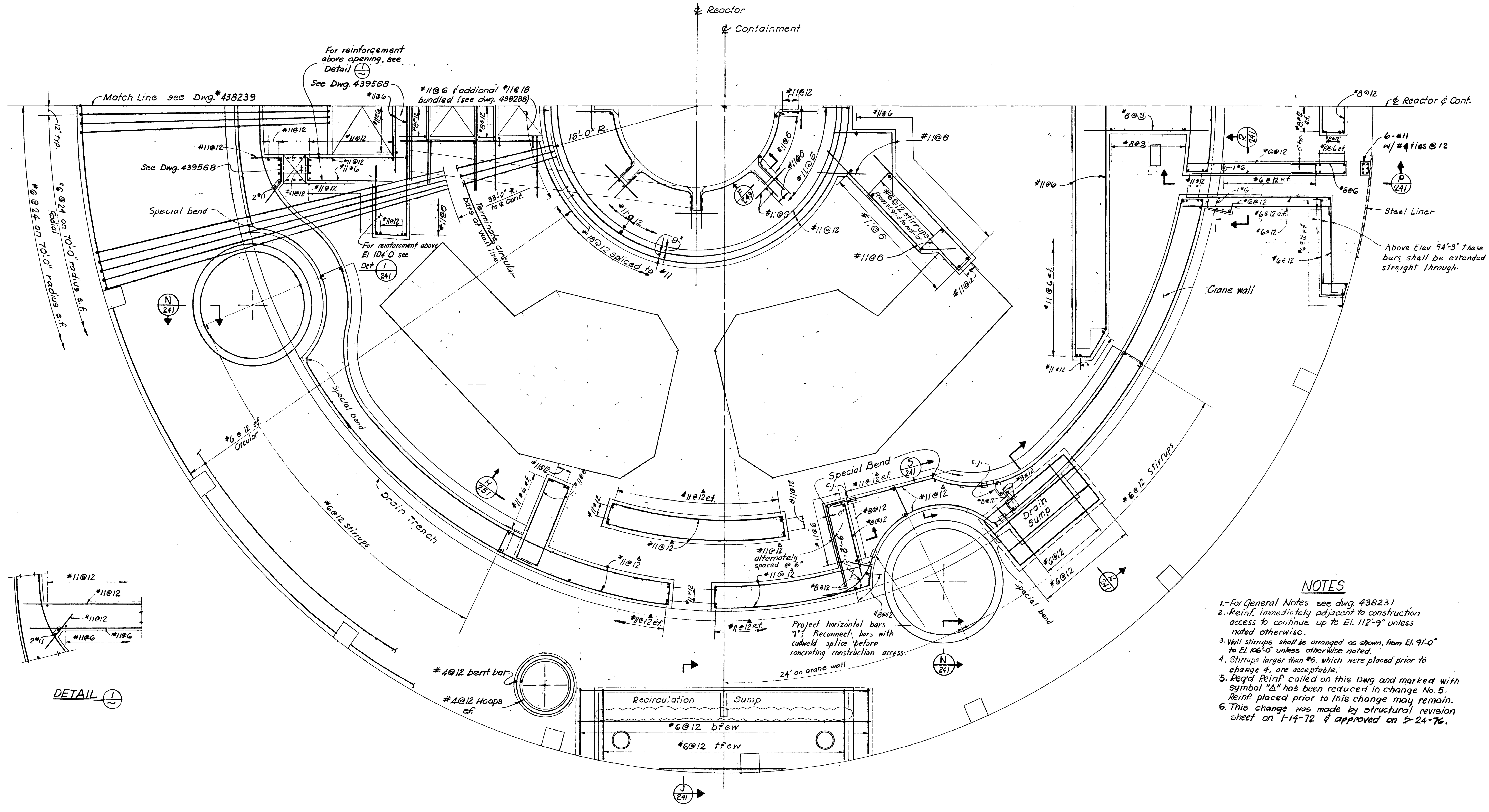
PLAN AT EL. 91'-0"
