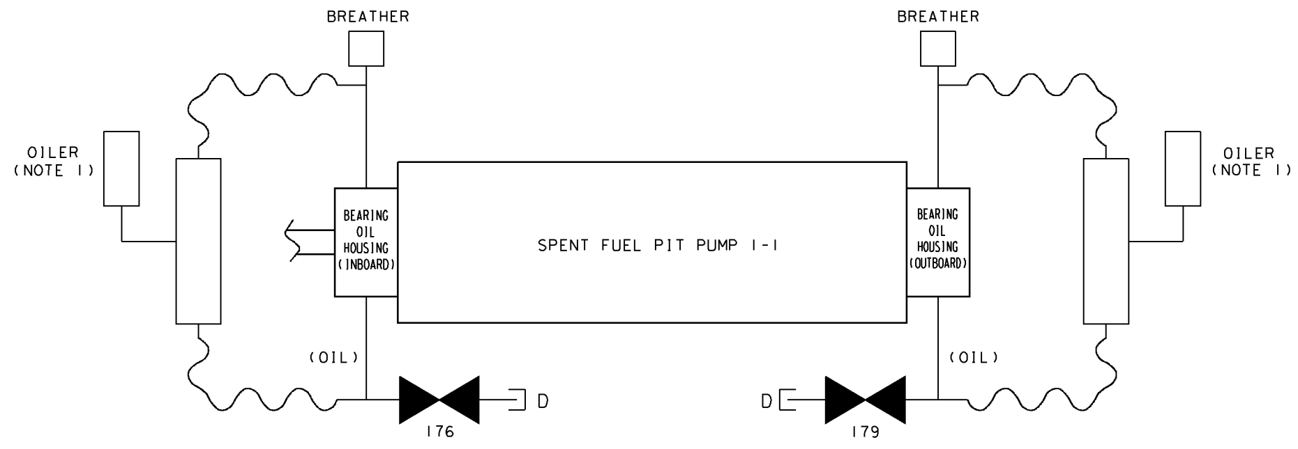
SPENT FUEL PIT PUMP 1-1 OIL LEVELIZER
