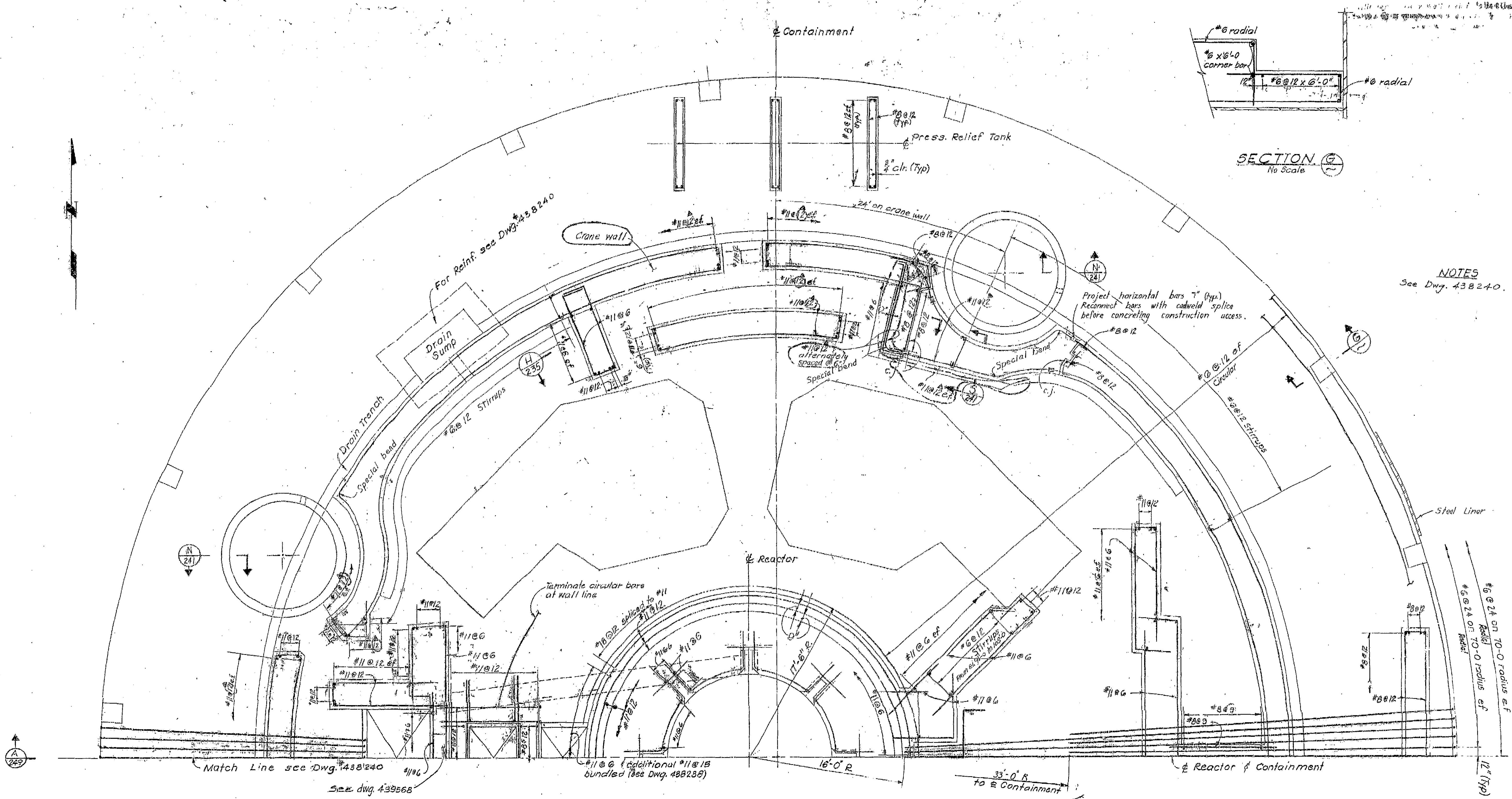
PLAN AT EL. 91'-0"
