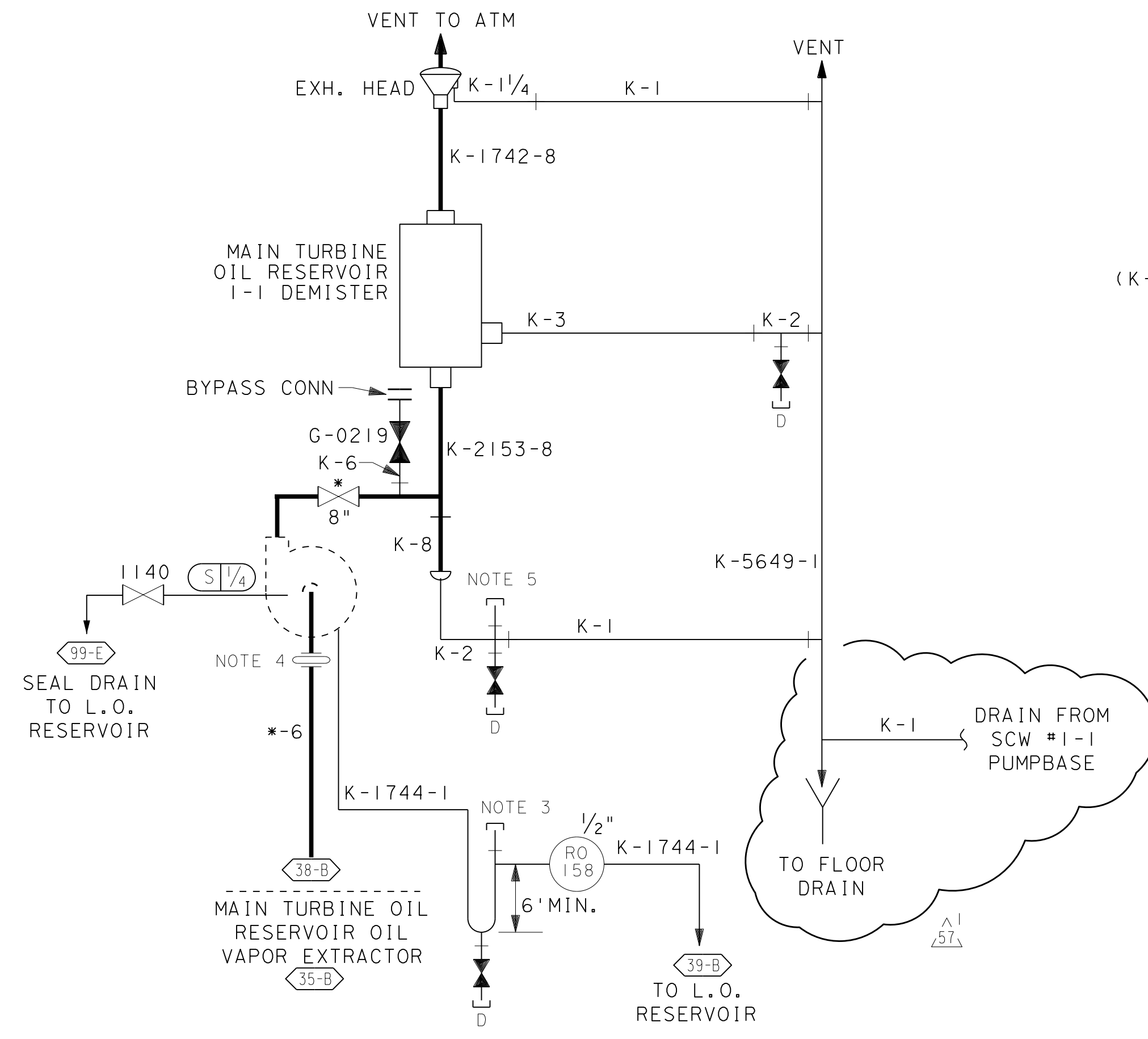
MAIN TURBINE OIL RESERVOIR VAPOR EXTRACTOR AND DEMISTER SYSTEM DC-663282-1
