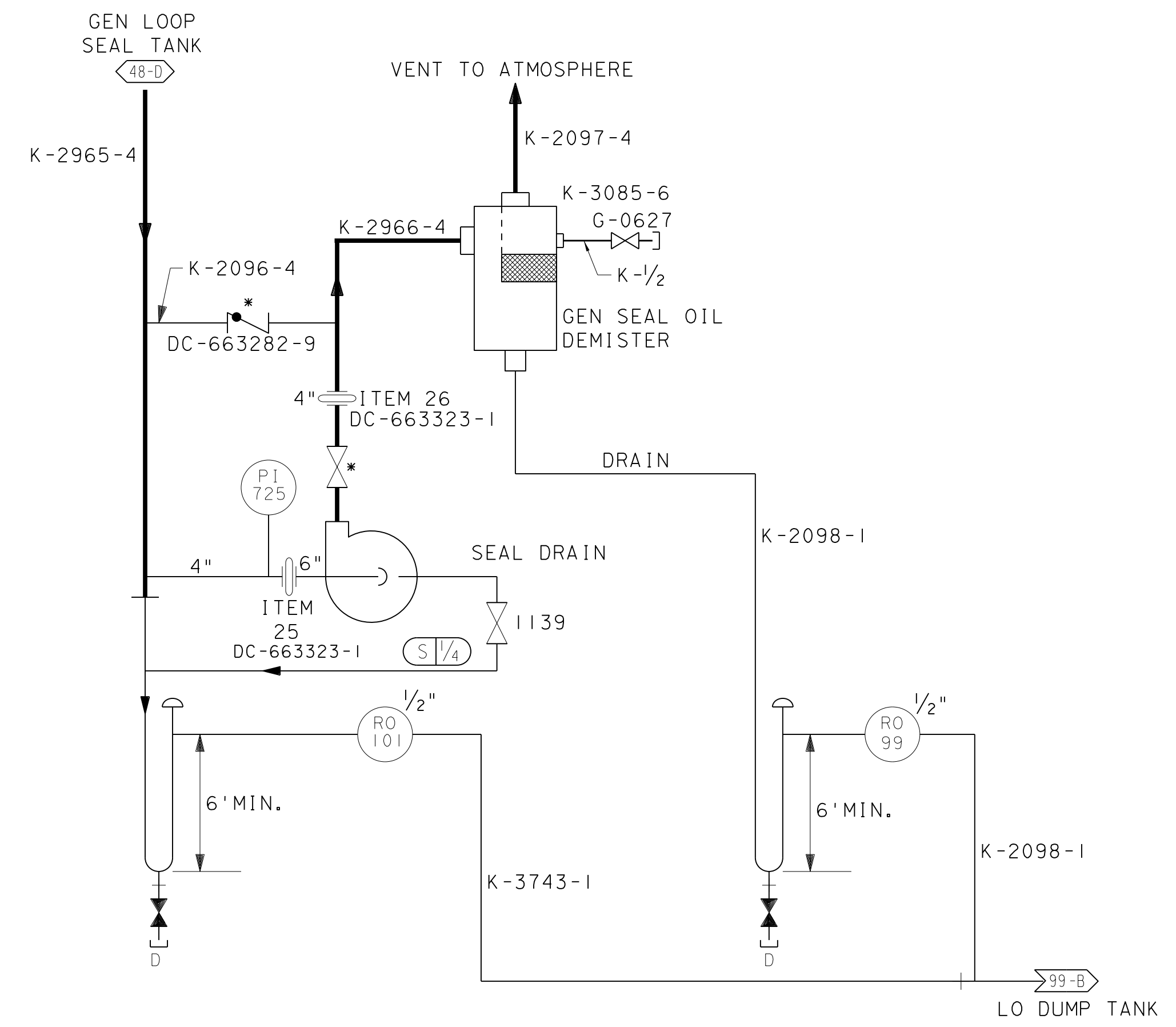
GENERATOR LOOP SEAL OIL TANK VAPOR EXTRACTOR AND DEMISTER SYSTEM DC-663282-3
