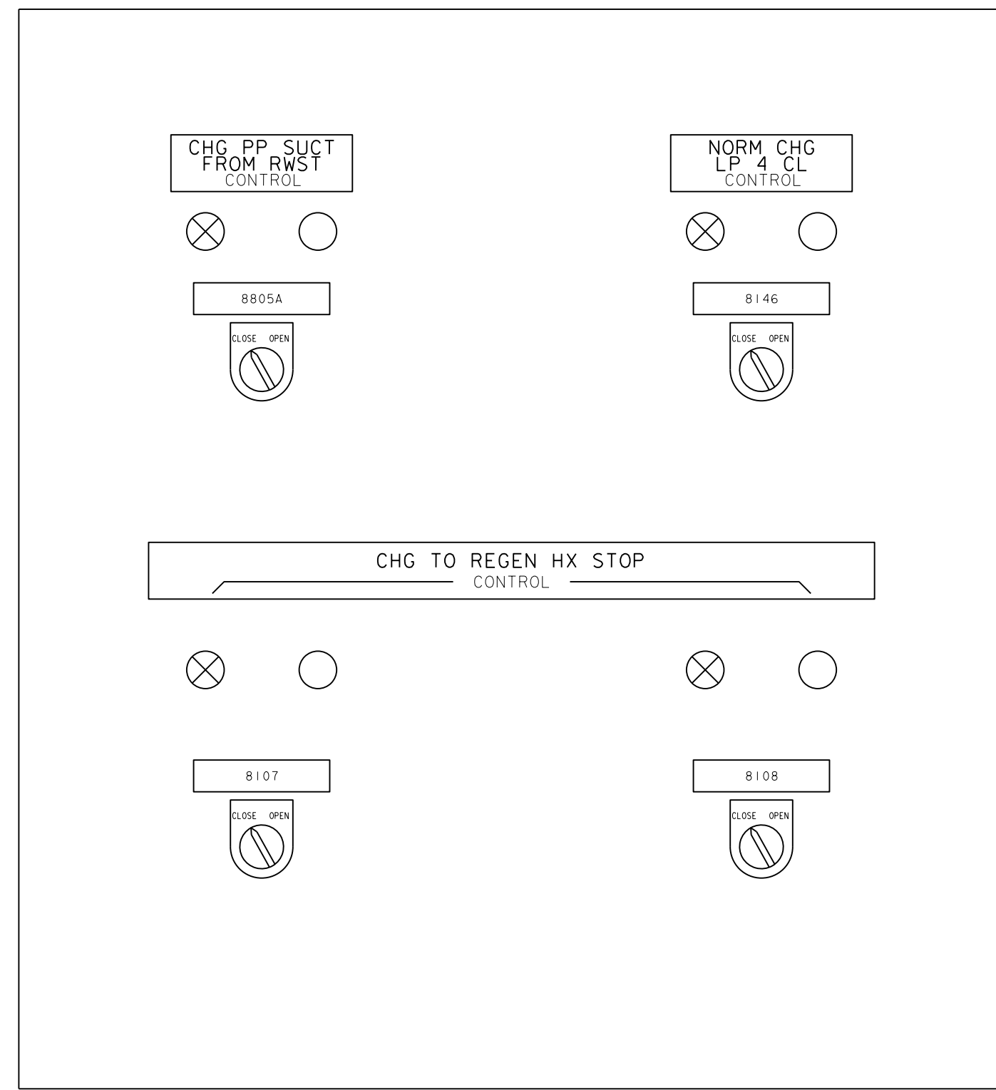
TOP PANEL
