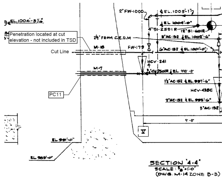
Figure 27 – Containment Wall Penetration Section 4-4 View (10588)
