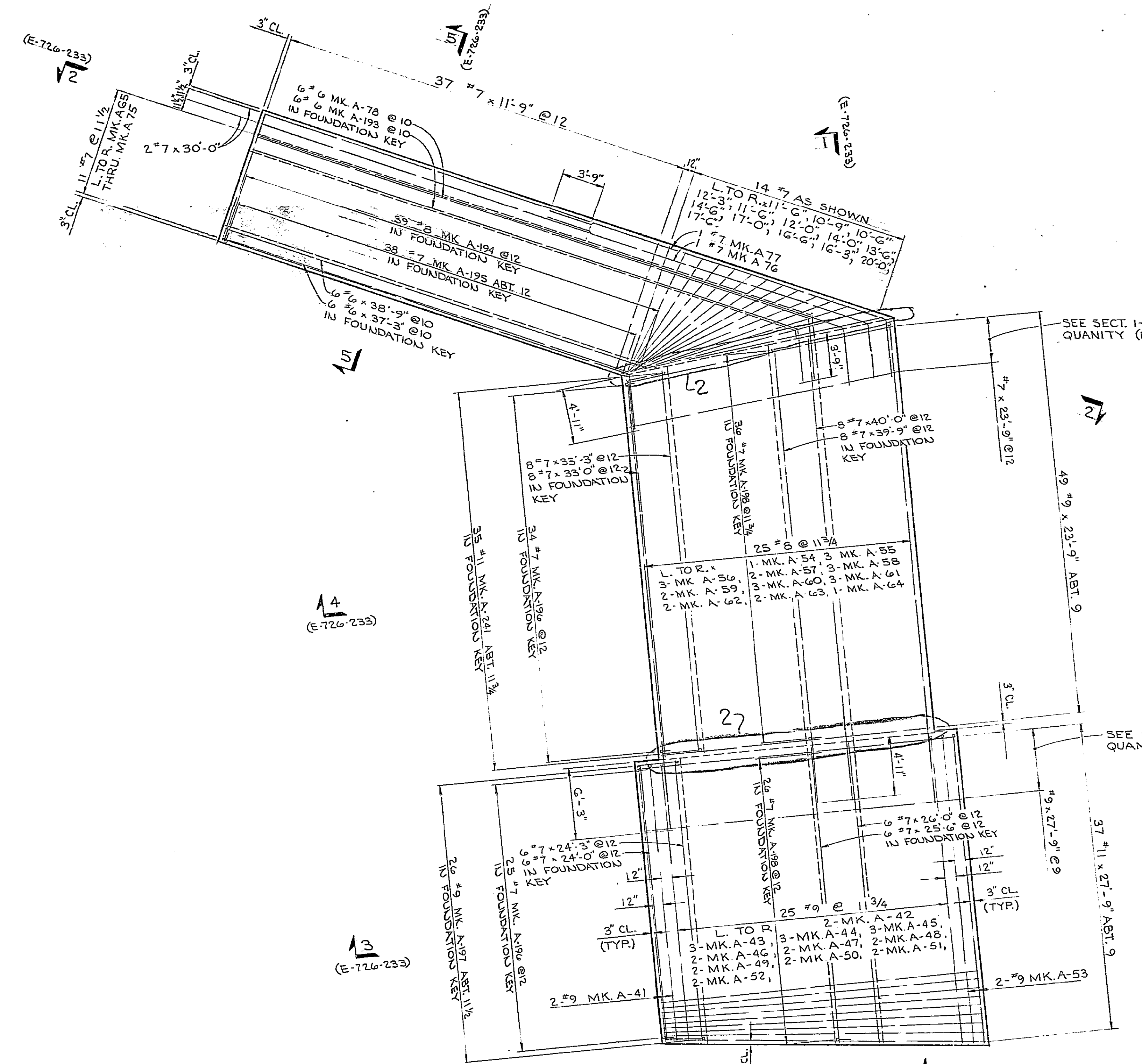
PLAN OF BOTTOM SLAB REINFORCEMENT RETAINING WALL NO. 1
