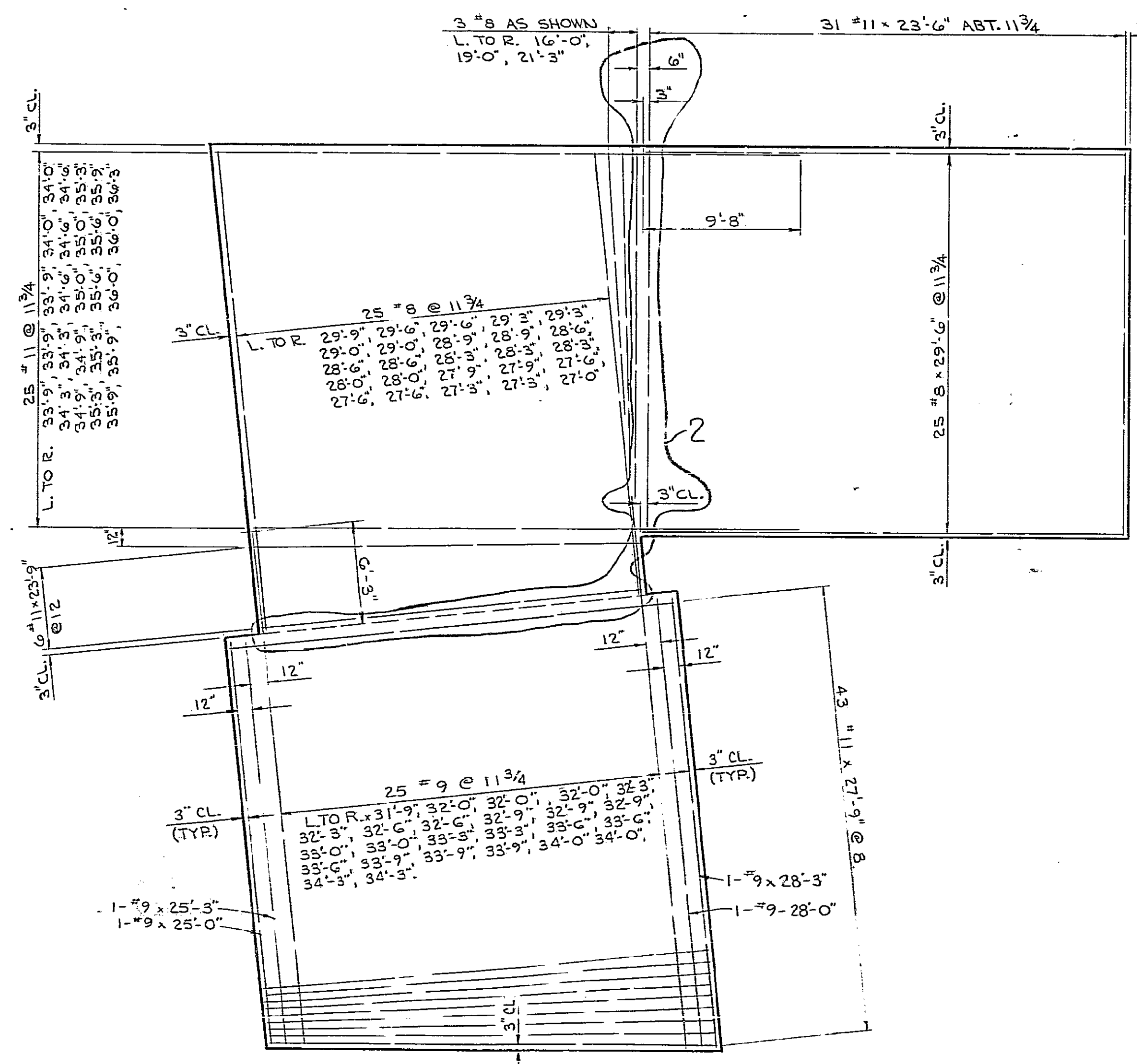
PLAN OF TOP SLAB REINFORCEMENT RETAINING WALL NO. 2
