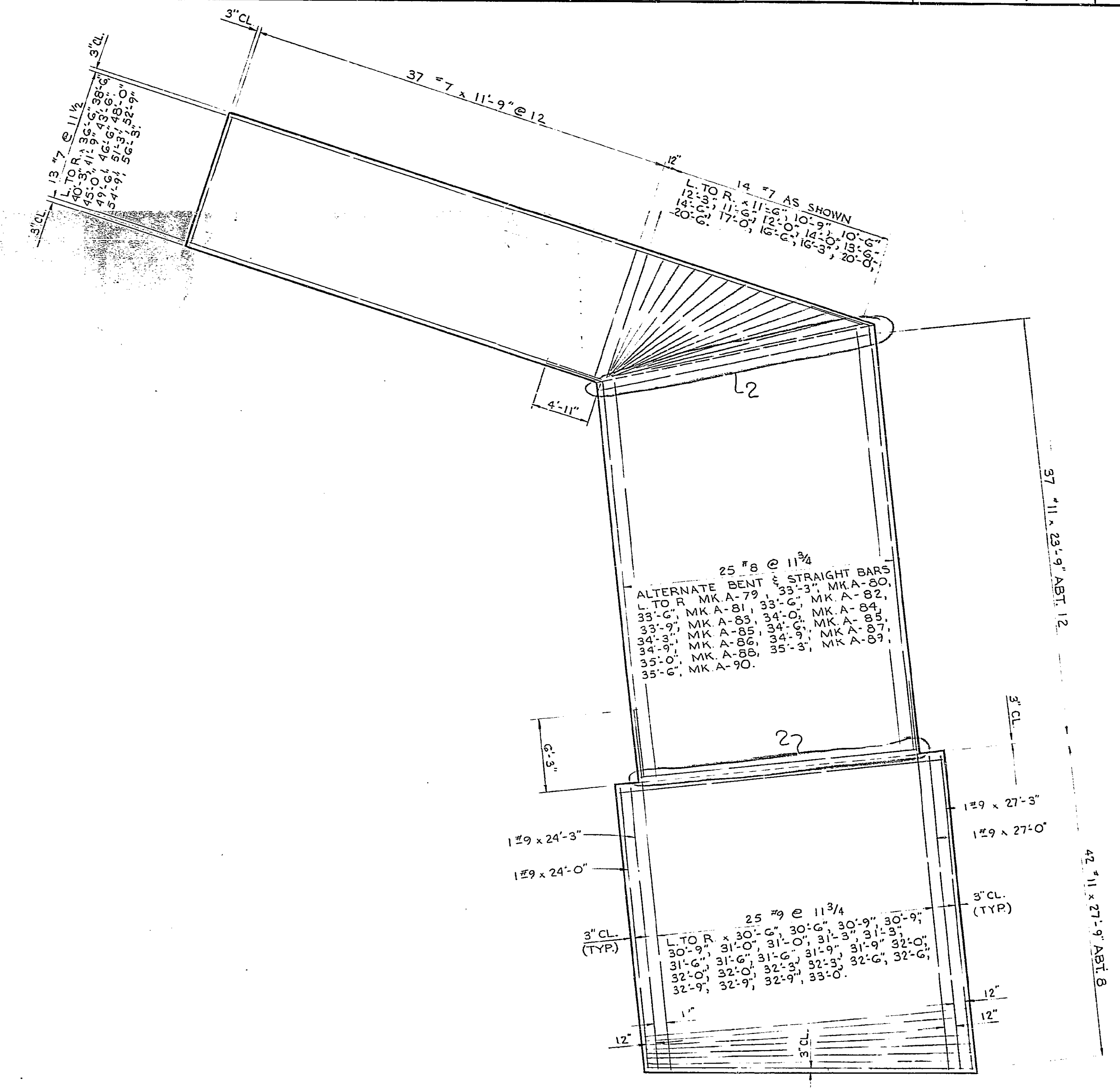
PLAN OF TOP SLAB REINFORCEMENT RETAINING WALL NO. 1
