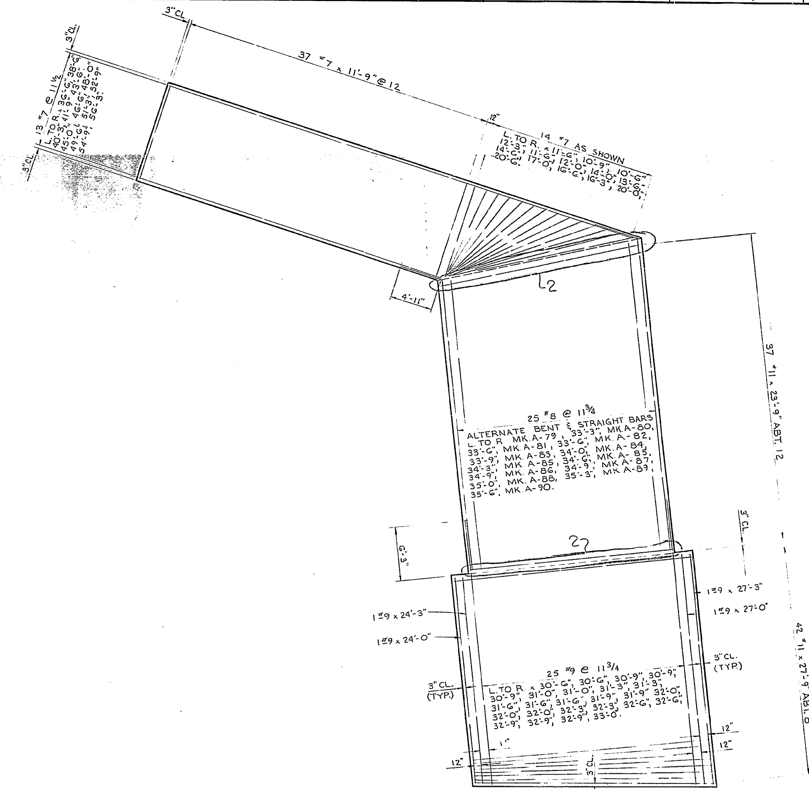
PLAN OF TOP SLAB REINFORCEMENT RETAINING WALL NO. 1
