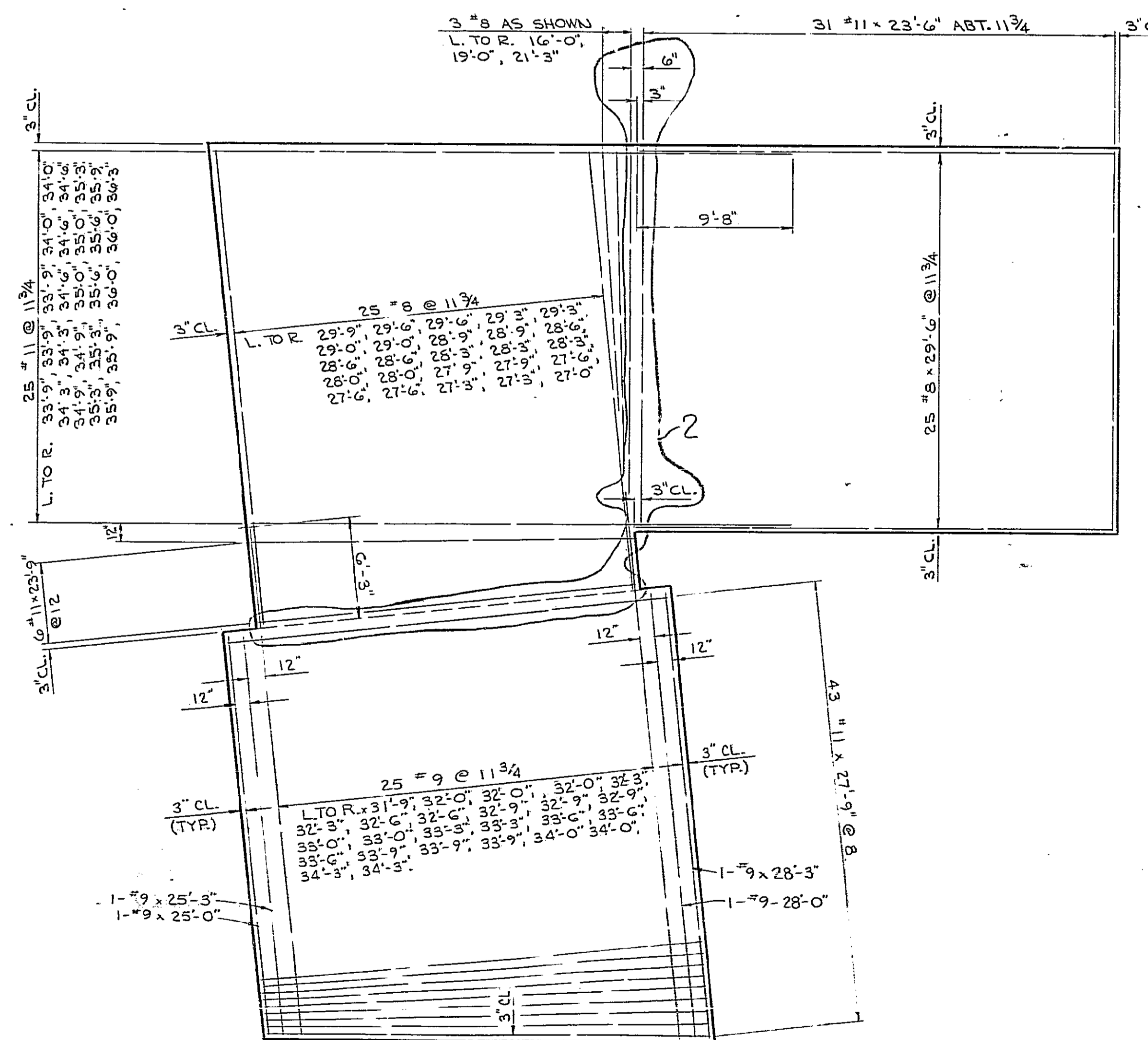
PLAN OF TOP SLAB REINFORCEMENT RETAINING WALL NO. 2
