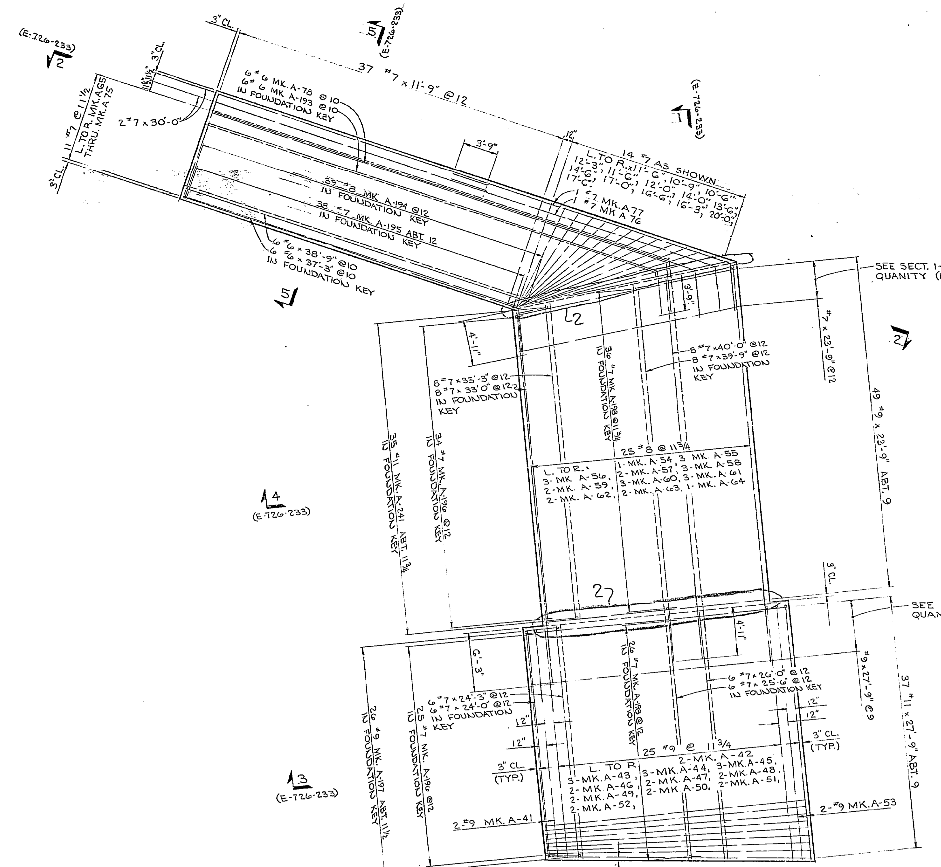
PLAN OF BOTTOM SLAB REINFORCEMENT RETAINING WALL NO. 1
