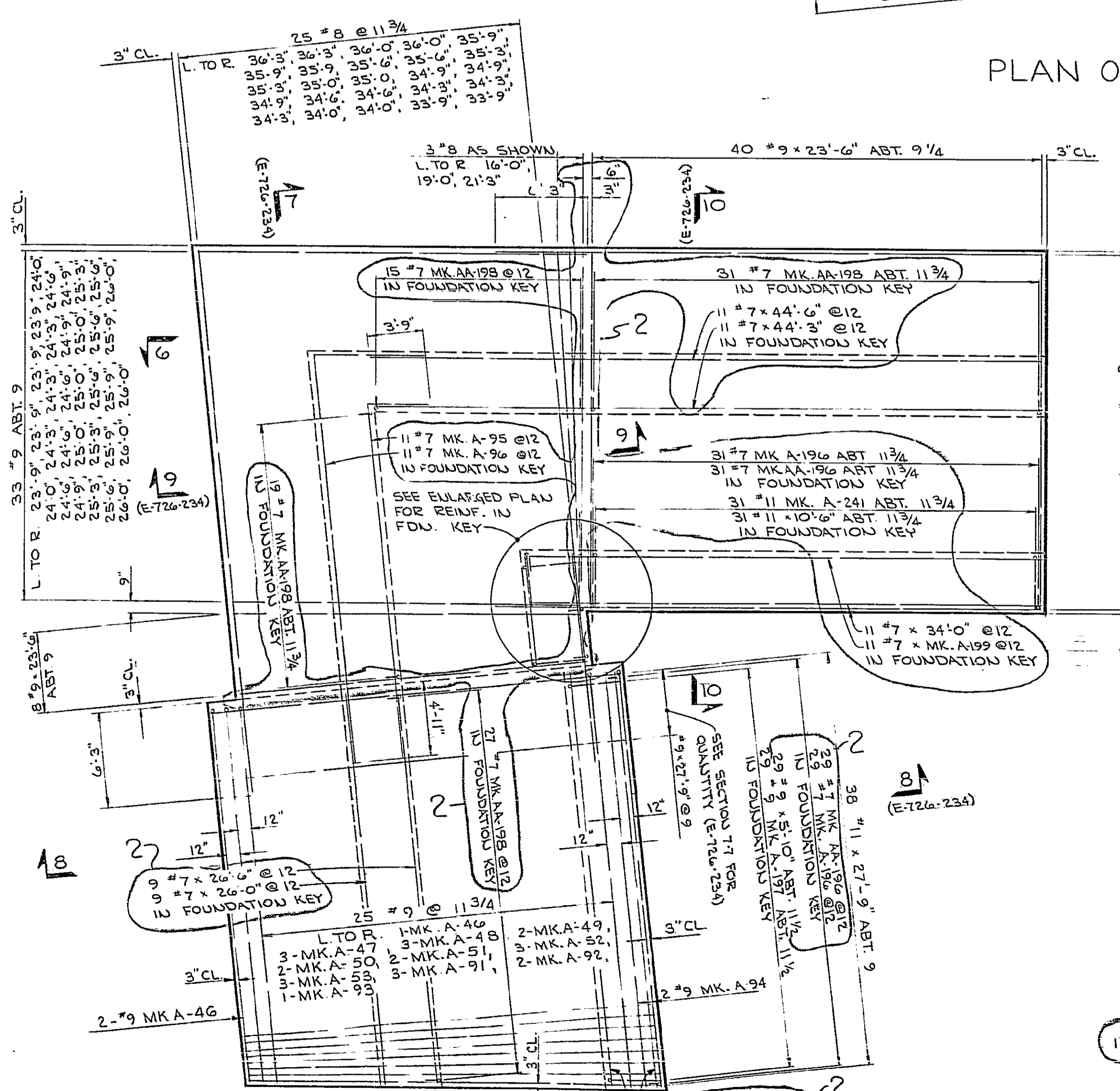
PLAN OF BOTTOM SLAB REINFORCEMENT RETAINING WALL NO. 2
