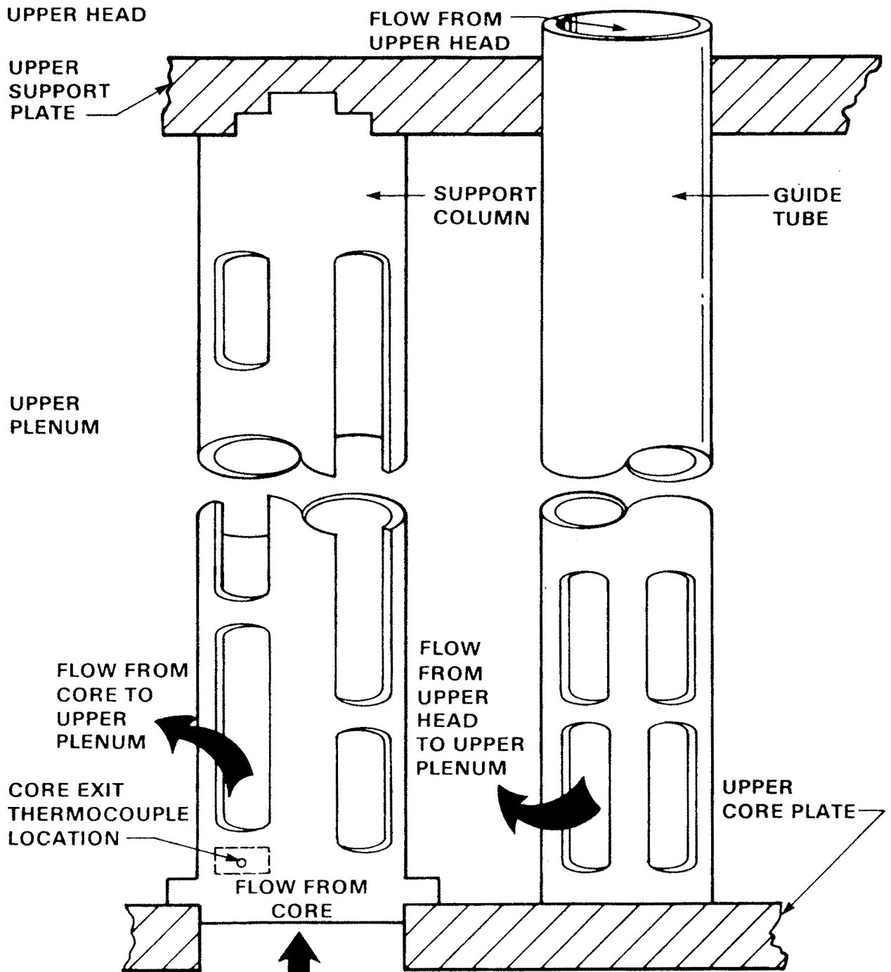
CALLAWAY PLANT Figure 492.28-1 Non-UHI Core Exit T/C Diagram
