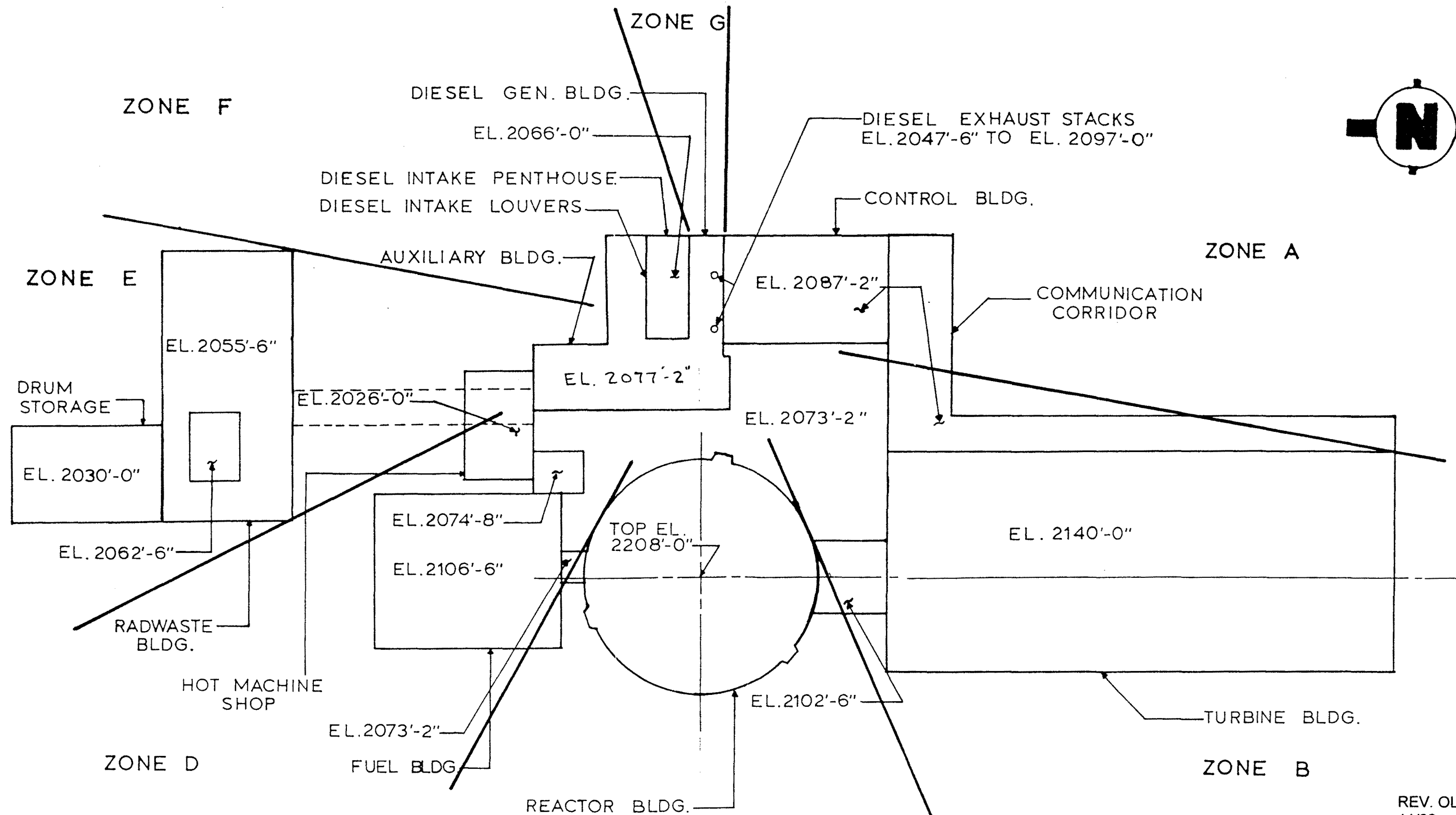
CALLAWAY PLANT FIGURE 430.38-1 STRUCTURAL PROTECTION FOR DIESEL EXHAUST STACKS FROM TORNADO MISSILES
