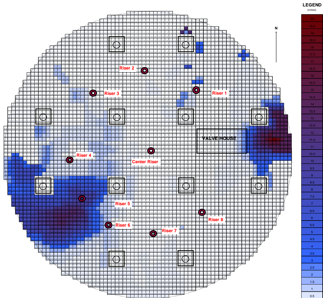
Figure 3.1-1: Tank 6 Residual Material Map
