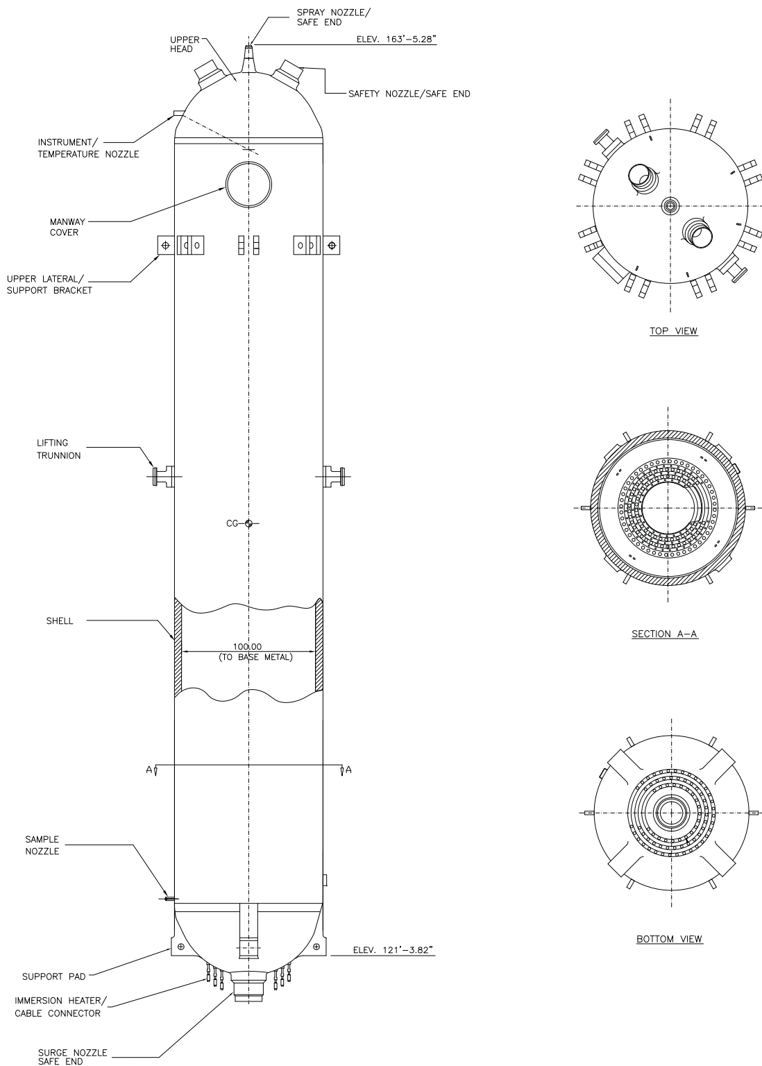
Figure 5.4-5 Pressurizer
