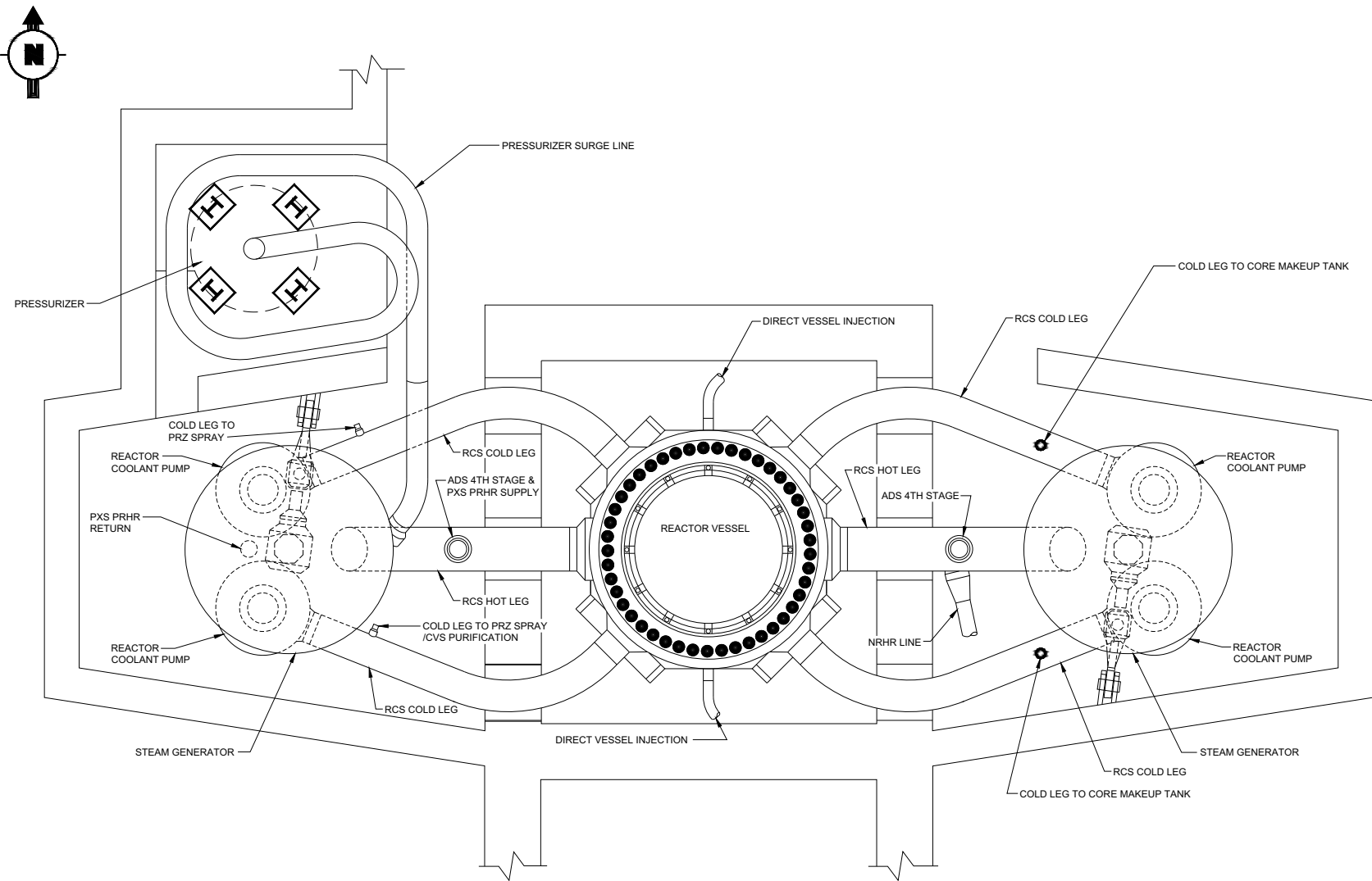
Figure 5.1-3 Reactor Coolant System – Loop Layout
