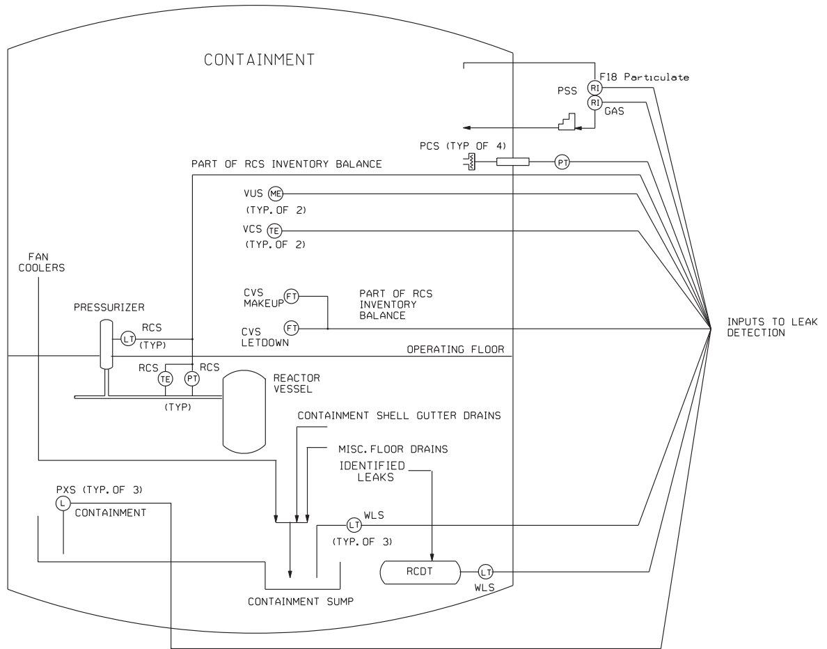
Figure 5.2-1 Leak Detection Approach
