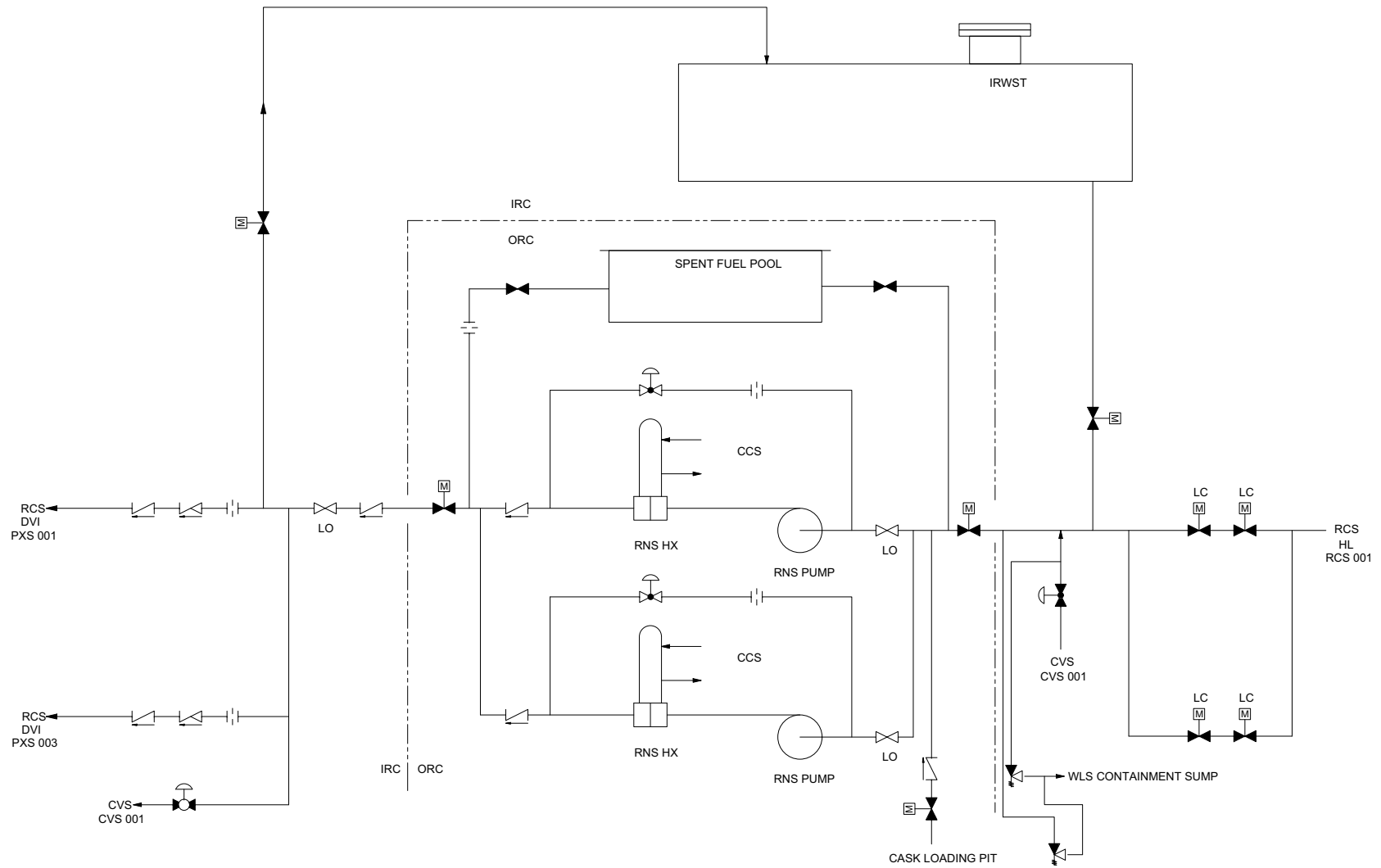
Figure 5.4-6 Normal Residual Heat Removal System
