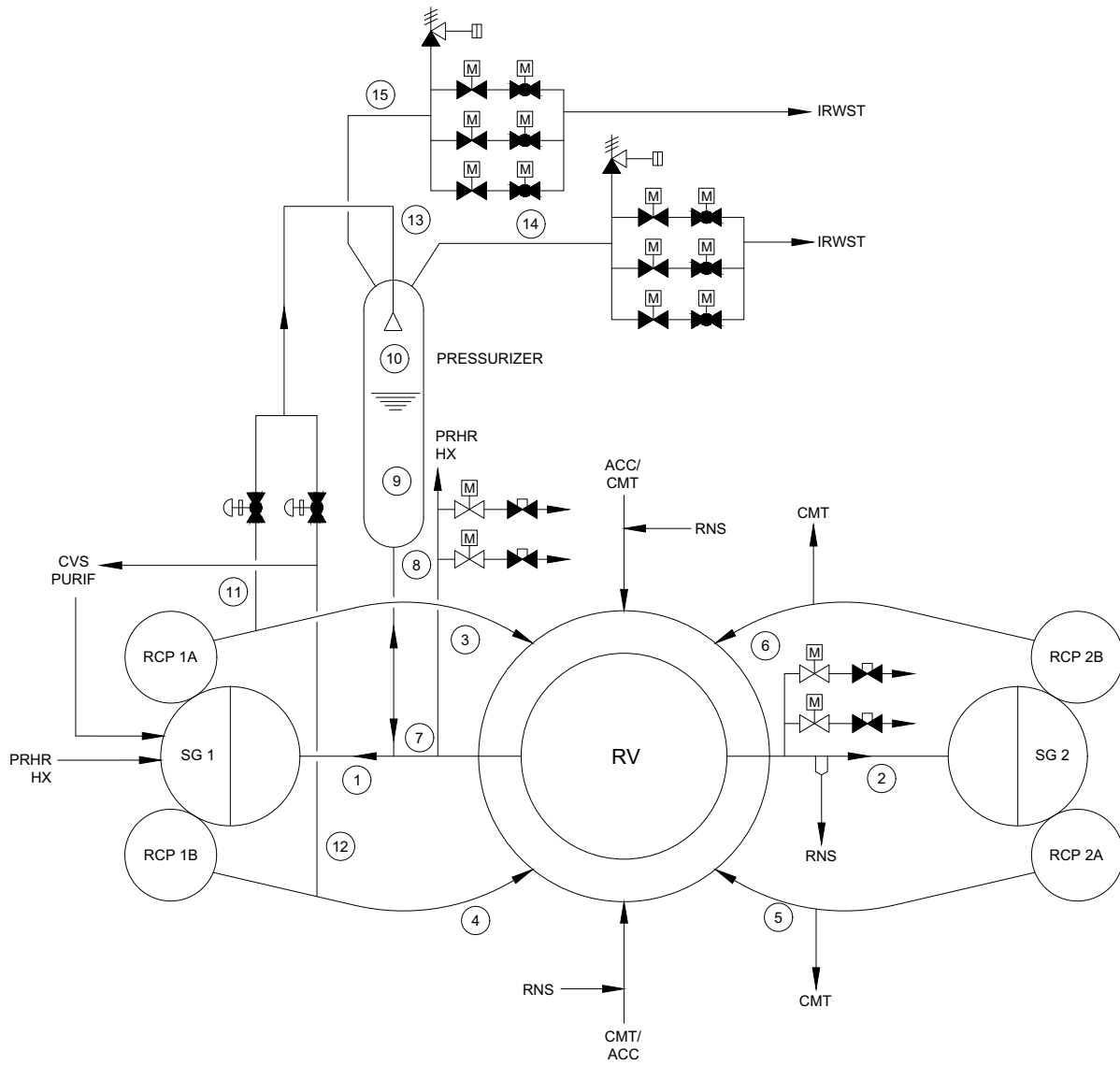
Figure 5.1-1 Reactor Coolant System Schematic Flow Diagram
