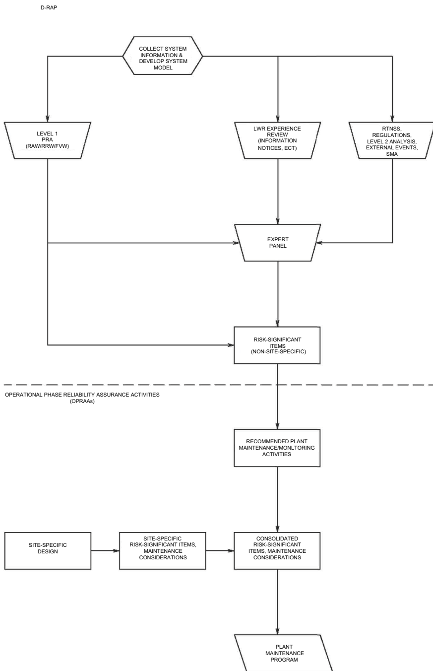
Figure 17.4-1 Design Reliability Assurance Program and Operational Phase Reliability Assurance Activities
