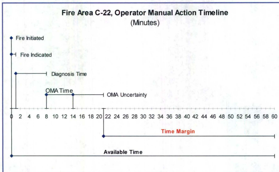
Figure 8.4.4-1, Fire Area C-22 OMA Timeline
