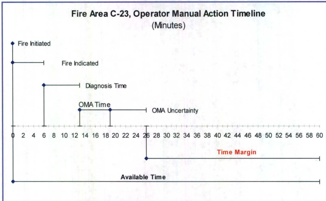
Figure 8.5.4-1, Fire Area C-23 OMA Timeline
