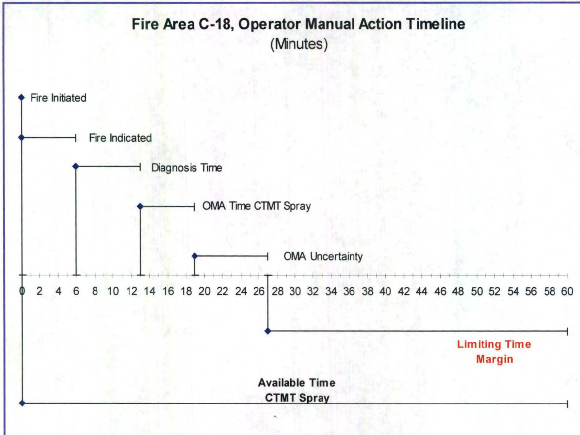
Figure 8.2.4-1, Fire Area C-18 OMA Timeline
