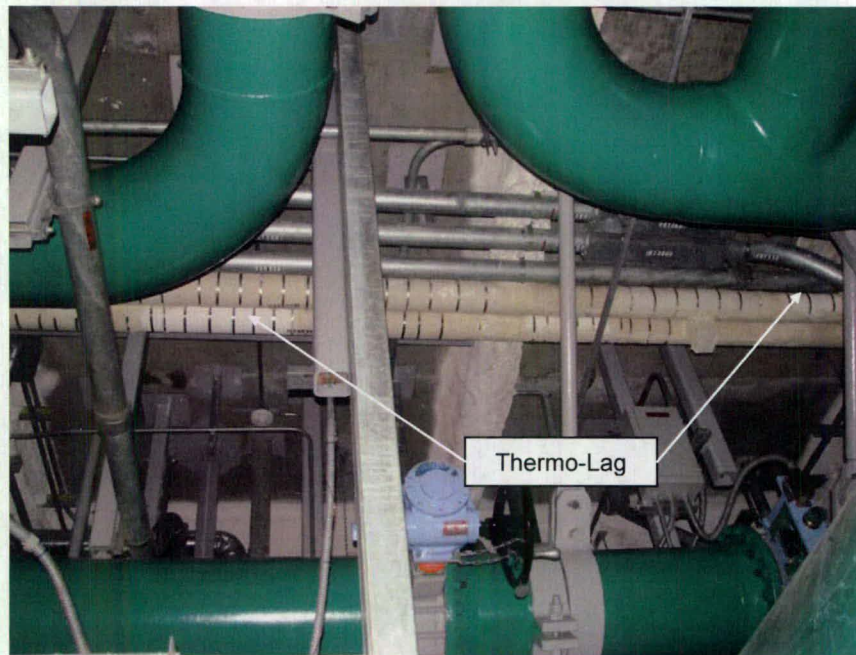
Photo 8.1.1-1, Typical Thermo-Lag IEEE-384 Protection
