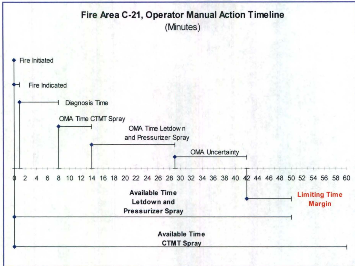
Figure 8.3.4-1, Fire Area C-21 OMA Timeline
