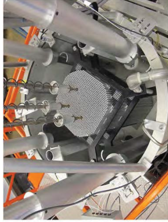
NCERC – Comet
