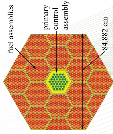
MOX3600
