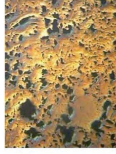
Nuclear Graphite
