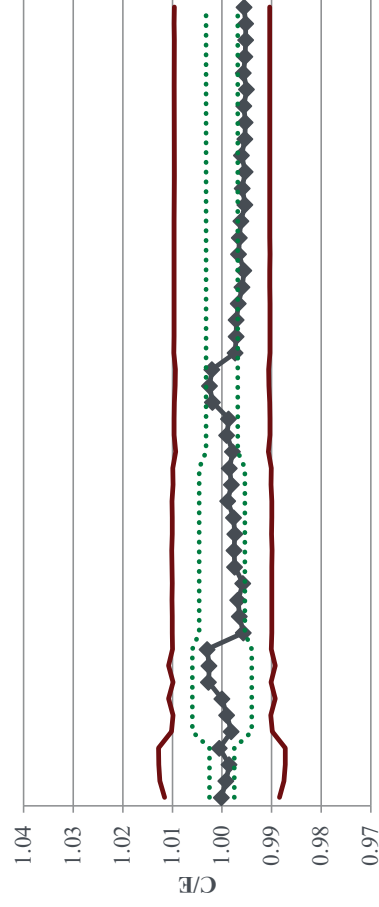
MIX-COMP-THERM
