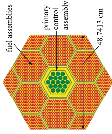
MET1000
