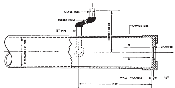
Figure F-2. Pipe cap orifice.
