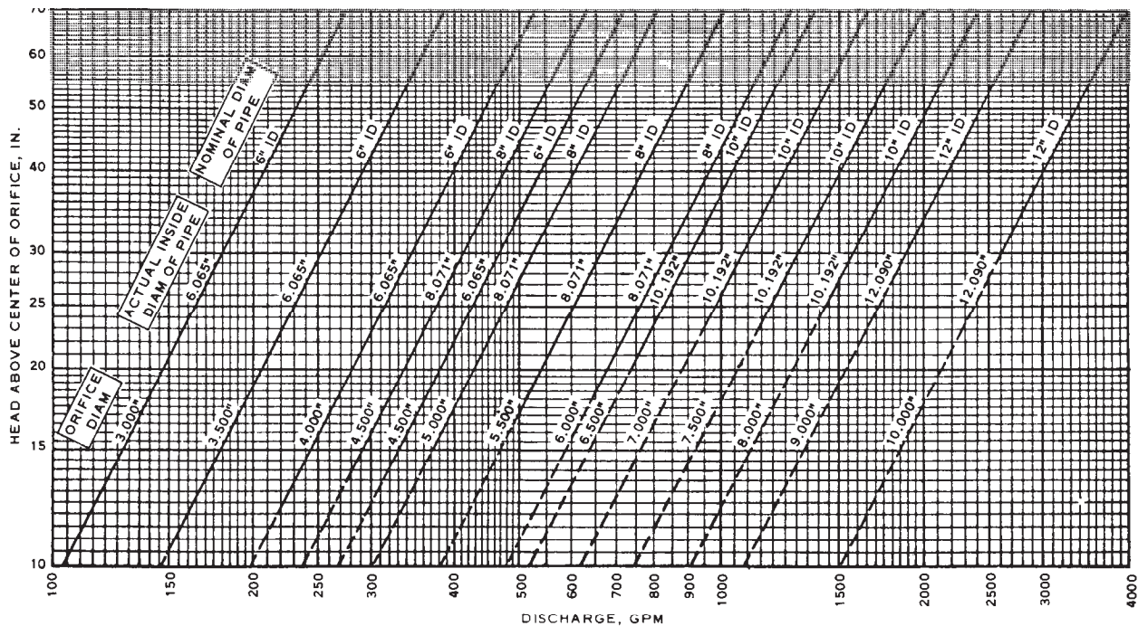
Figure F-5. Pipe cap orifice chart.
