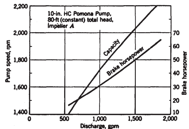
Figure 4-35. Rating curves for a three-stage 10-inch-high capacity deep-well pump.
