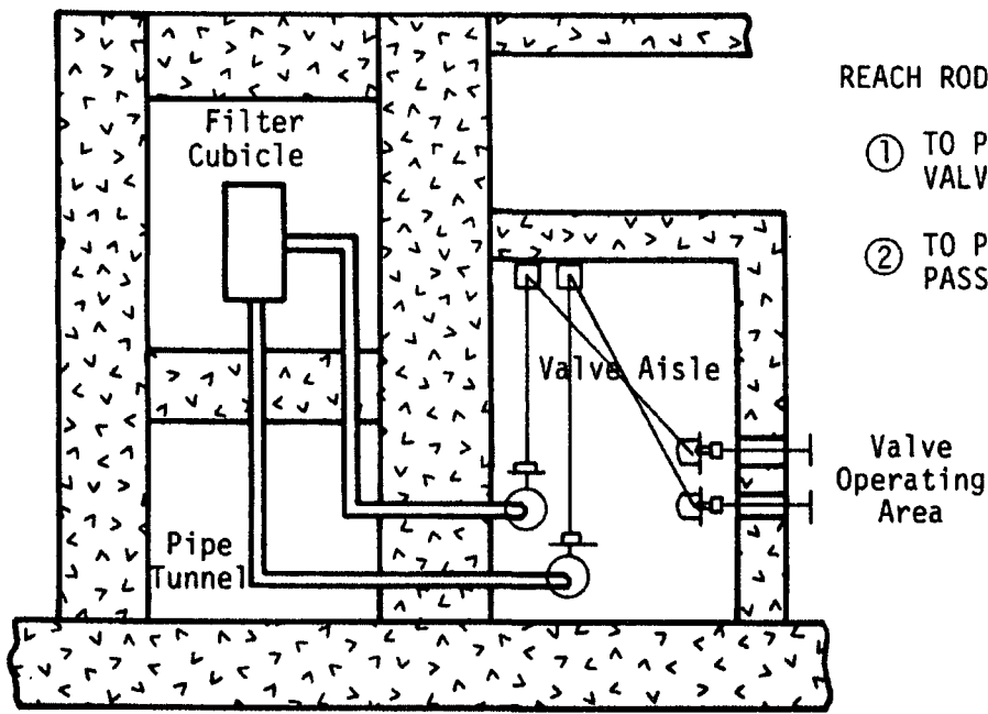
WALK-IN VALVE AISLE (ELEVATION)
