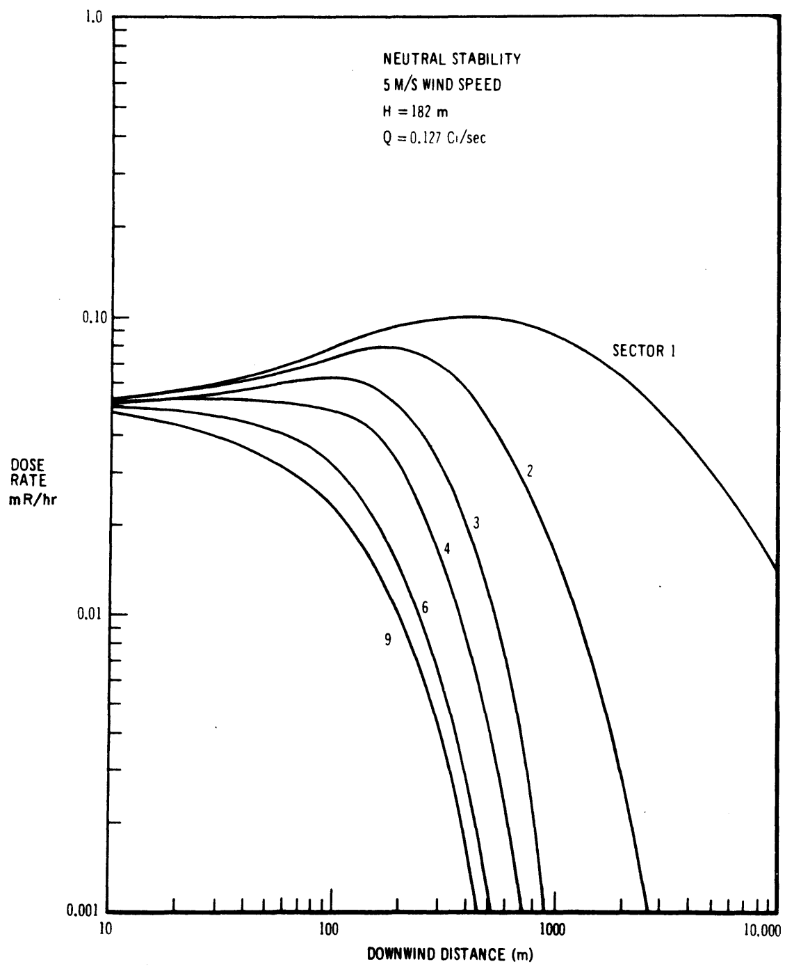
PHILADELPHIA ELECTRIC COMPANY PEACH BOTTOM ATOMIC POWER STATION UNITS 2 AND 3 UPDATED FINAL SAFETY ANALYSIS REPORT DOSE RATE IN EACH SECTOR FIGURE E.2.3
