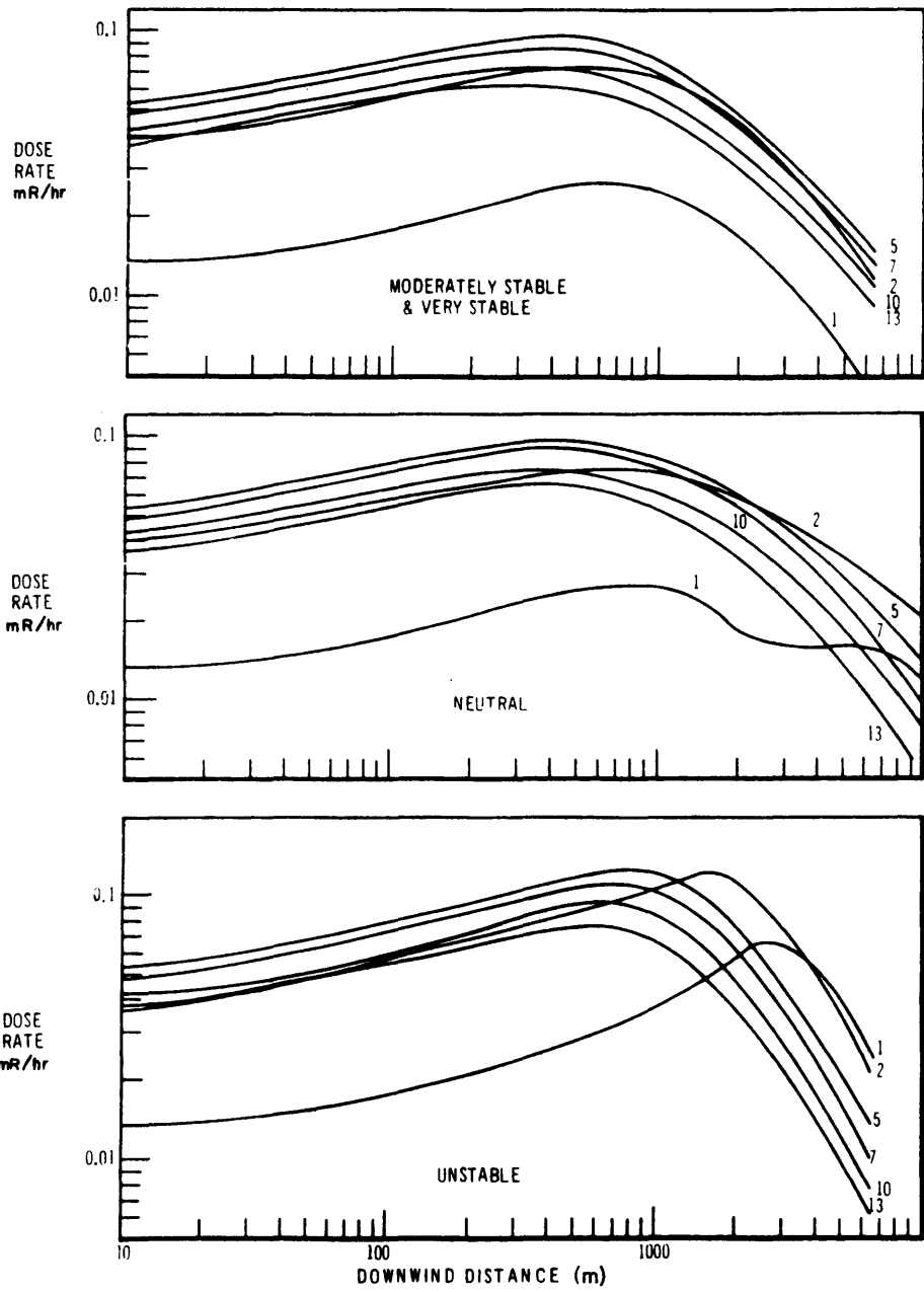
PHILADELPHIA ELECTRIC COMPANY PEACH BOTTOM ATOMIC POWER STATION UNITS 2 AND 3 UPDATED FINAL SAFETY ANALYSIS REPORT GAMMA DOSE RATE FOR VARIOUS WIND SPEEDS AND STABILITIES FOR BGRR STACK (RELEASE RATE 0.127 Ci/sec) FIGURE E.2.1
