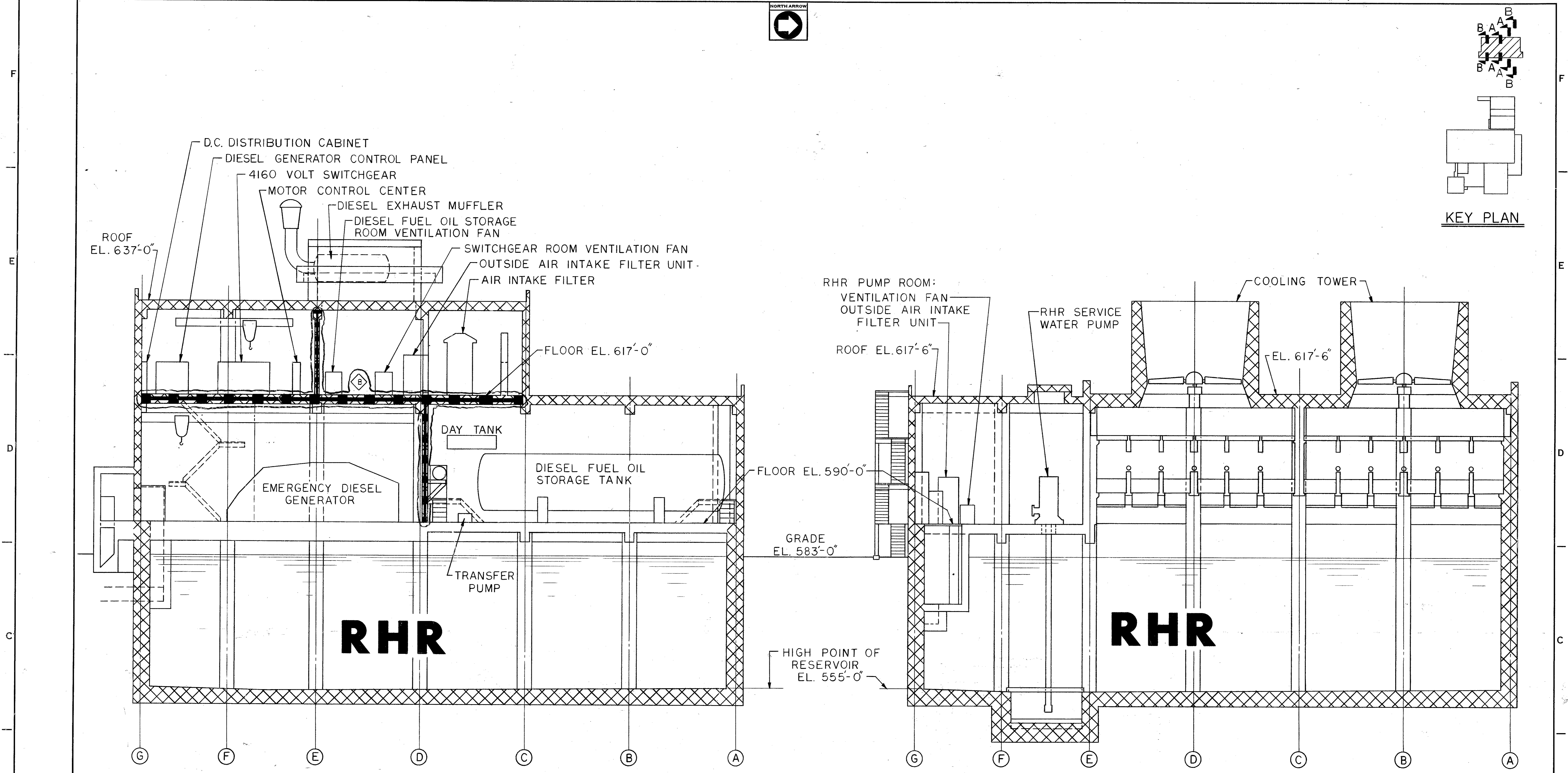
TYPICAL SECTION A-A LOOKING SOUTH DIVISION 1-DIVISION 2
