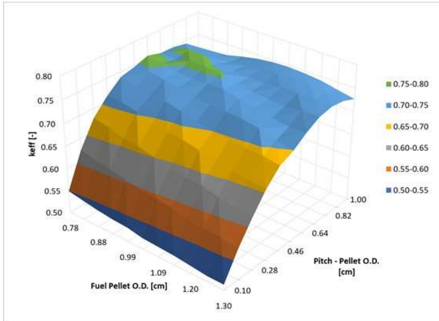
Figure 11. Rod pipe model k_{eff} for fuel pellet OD and rod pitch combinations for 5 wt.% \text{UO}_2 .
