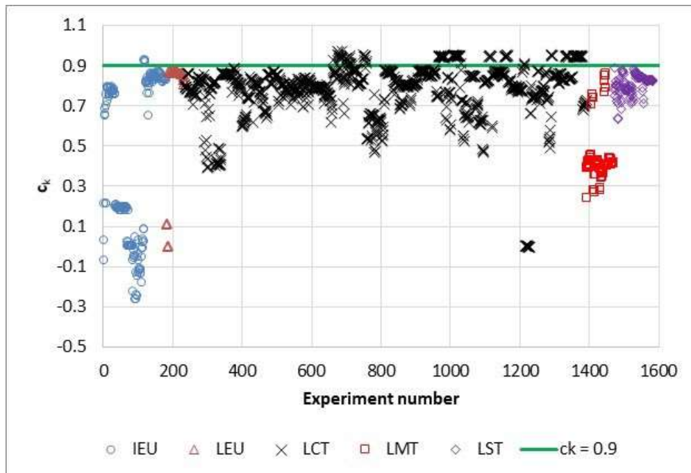
Figure 27. CHT-OP-TU c_k for 16.5 wt.% \text{UO}_2 pellets (48 packages, 6 in. diameter OV).
