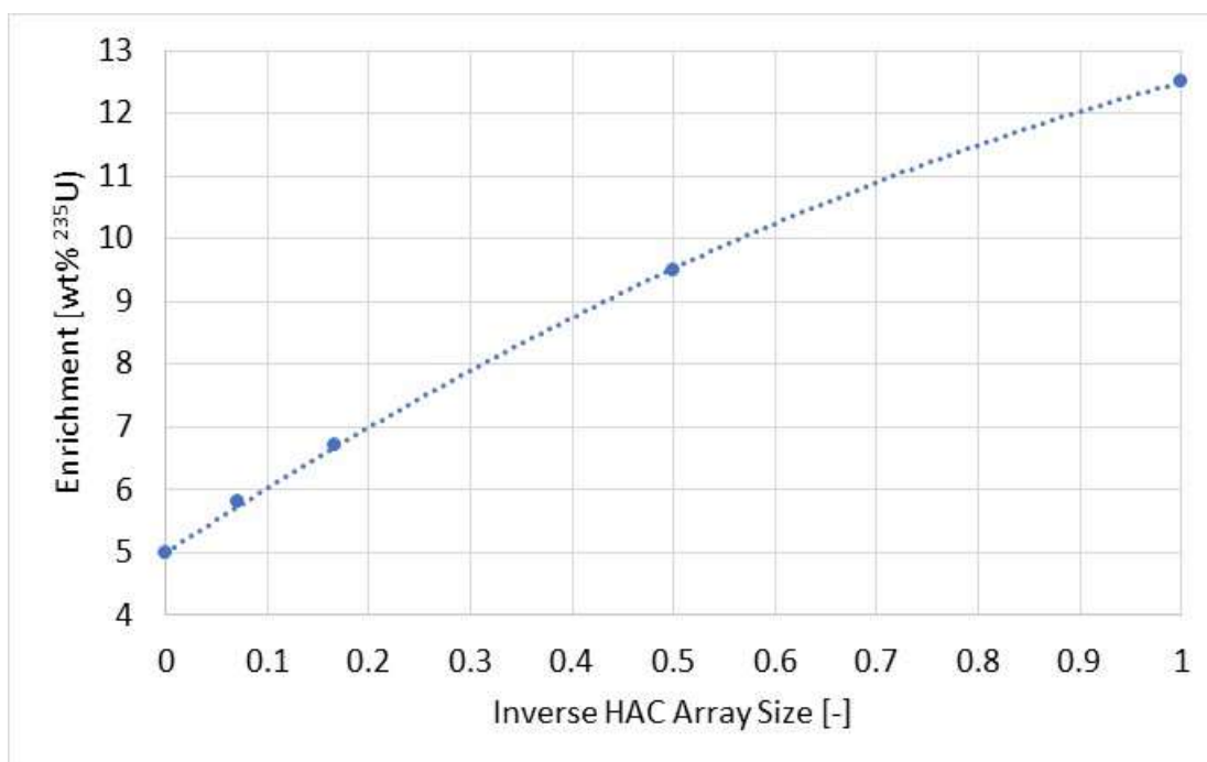
Figure 45. DN-30 model enrichment and array size.
