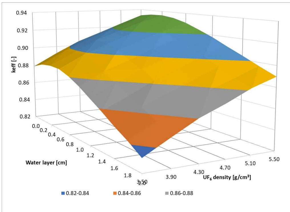
Figure 43. DN-30 3 x 2 HAC array k_{eff} .
