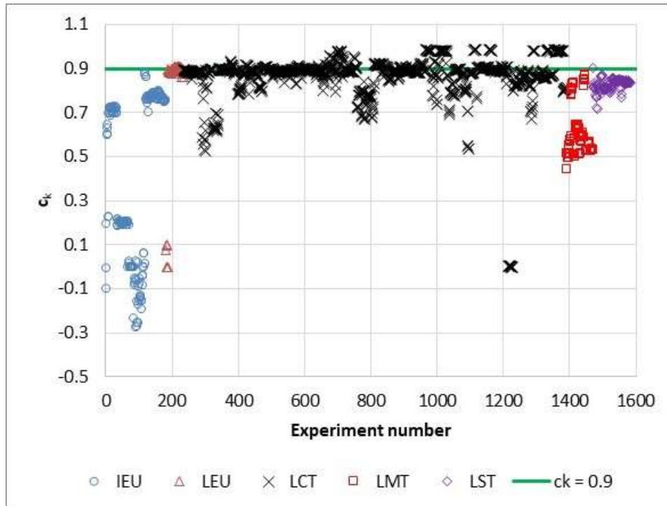
Figure 22. CHT-OP-TU c_k for 5 wt.% UO 2 powder (48 packages, 8 in. diameter OV).
