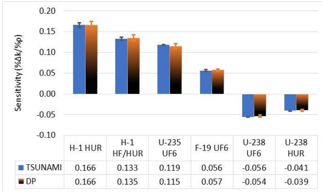
Figure 47. DN-30 model sensitivity (6.7 wt.%, 3 \times 2 array).
