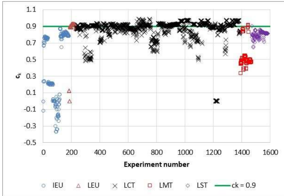
Figure 26. CHT-OP-TU c_k for 6.9 wt.% \text{UO}_2 pellets (18 packages, 7.5 in. diameter OV).
