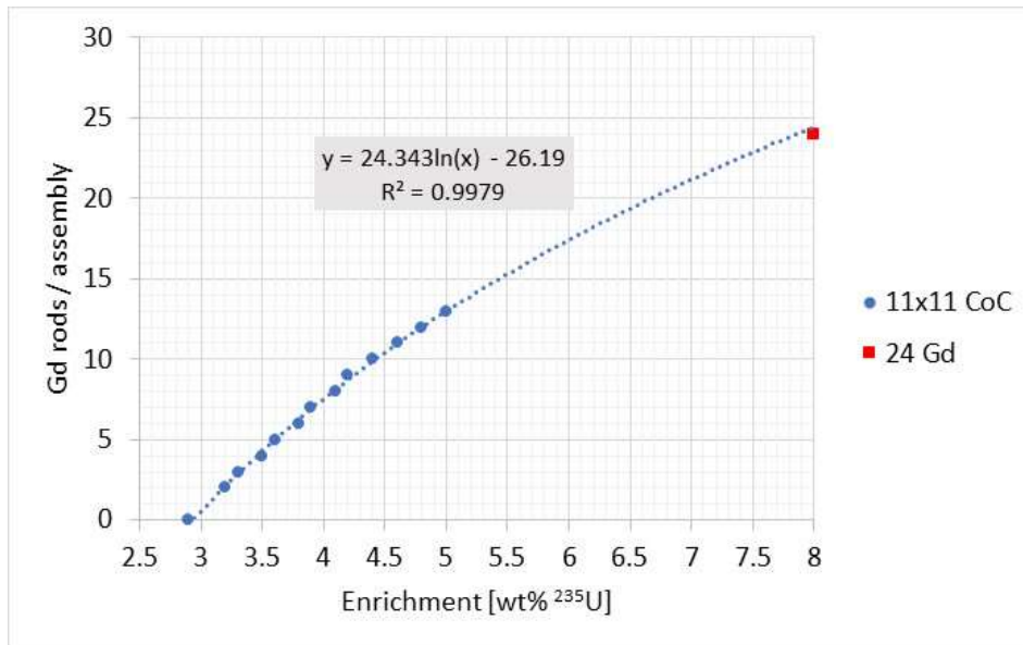
Figure 33. TN-B1 10 \times 1 \times 10 package Gd rods required vs. fuel assembly enrichment.
