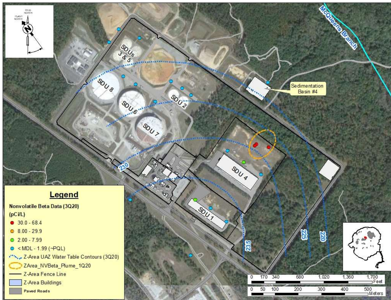
Figure 10. Approximate Nonvolatile Beta Groundwater Plume (3Q20)
