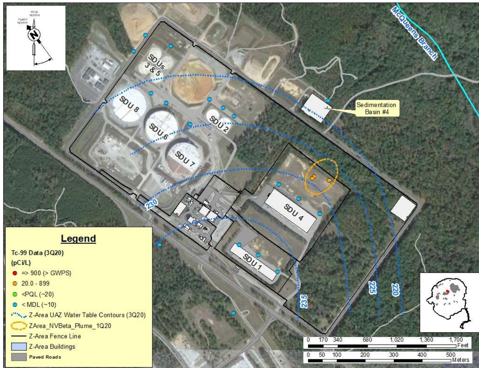
Figure 12. Approximate Tc-99 Groundwater Plume (3Q20)
