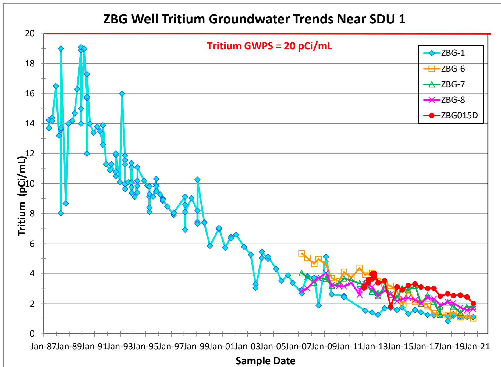
Figure 14. ZBG Well Tritium Groundwater Trends
