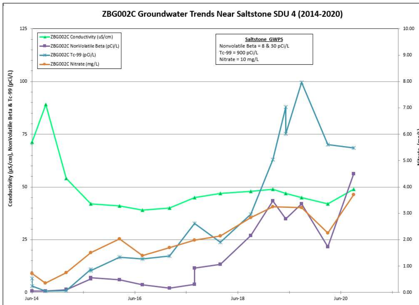
Figure 11. ZBG002C Groundwater Trends
