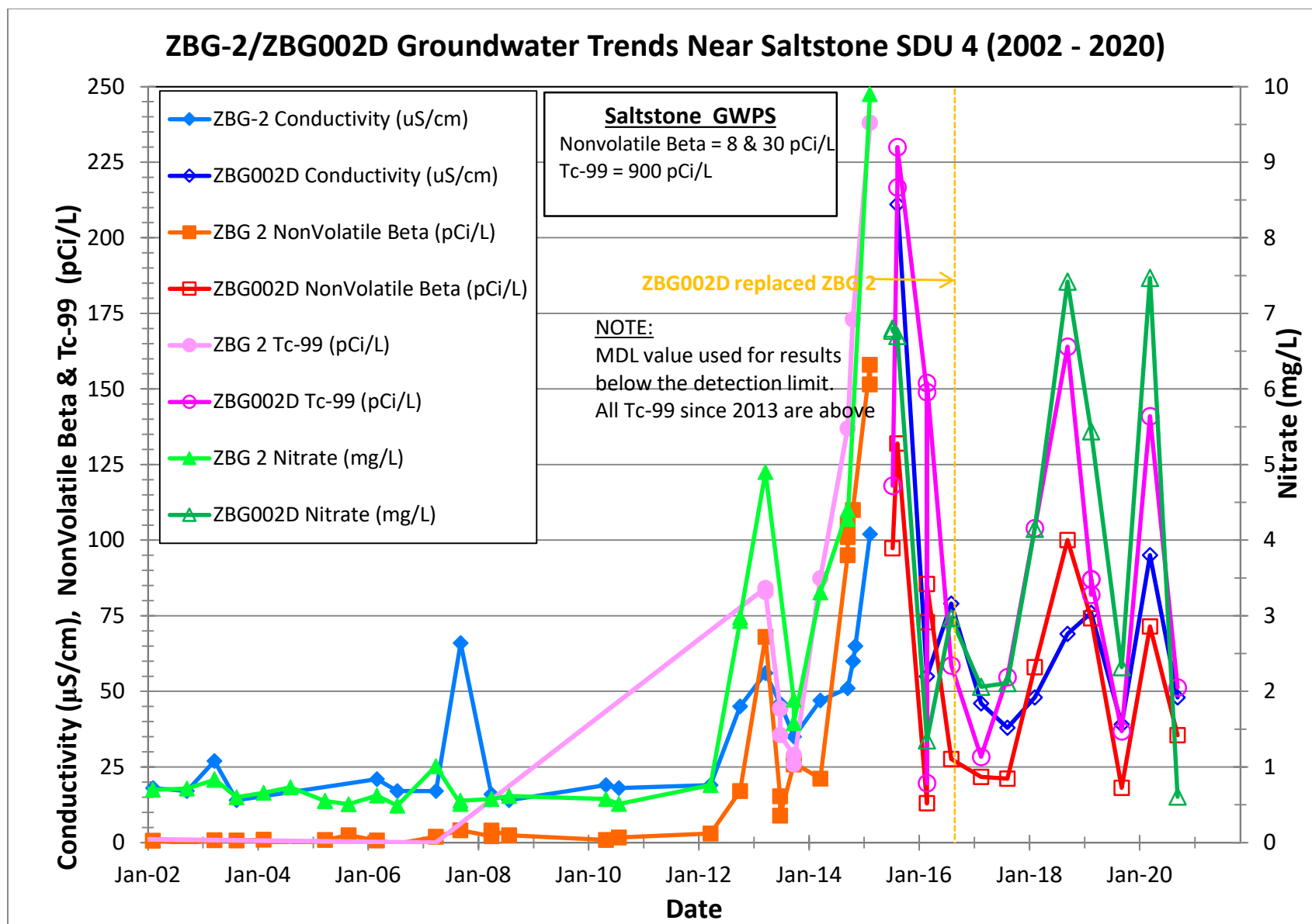
Figure 9. ZBG 2 / ZBG002D Tc-99 Groundwater Trends
