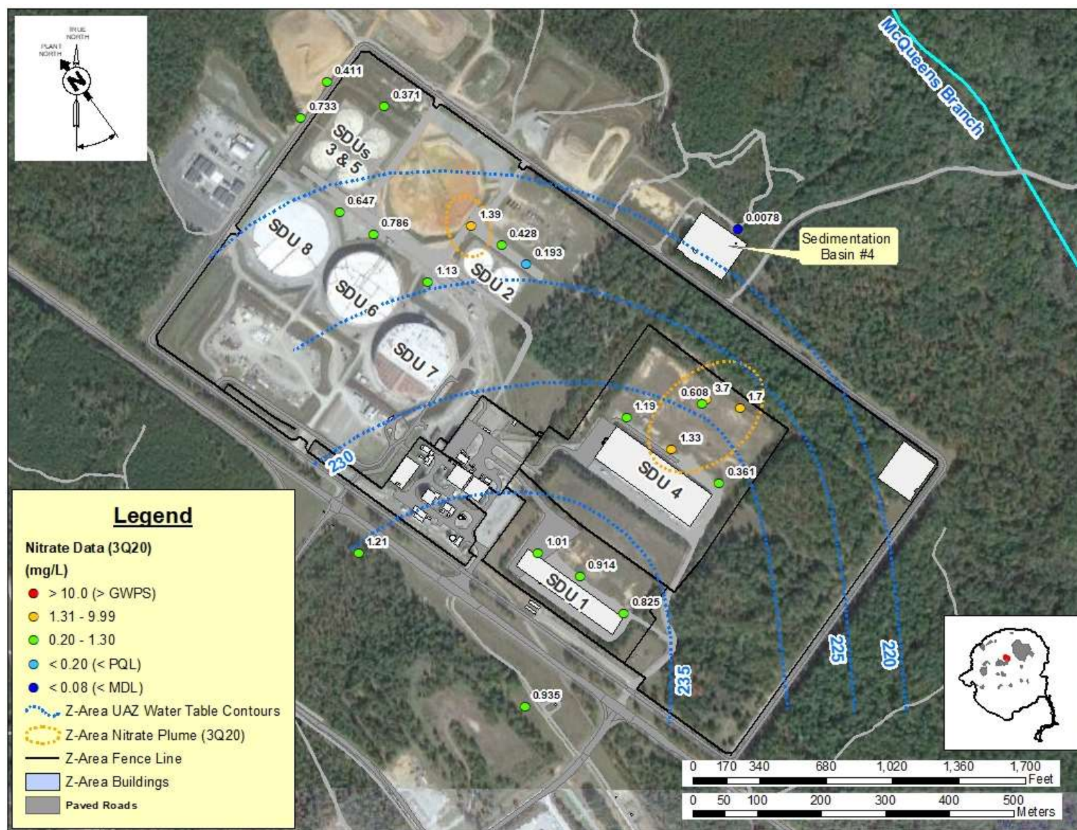
Figure 13. Approximate Nitrate Groundwater Plume (3Q20)
