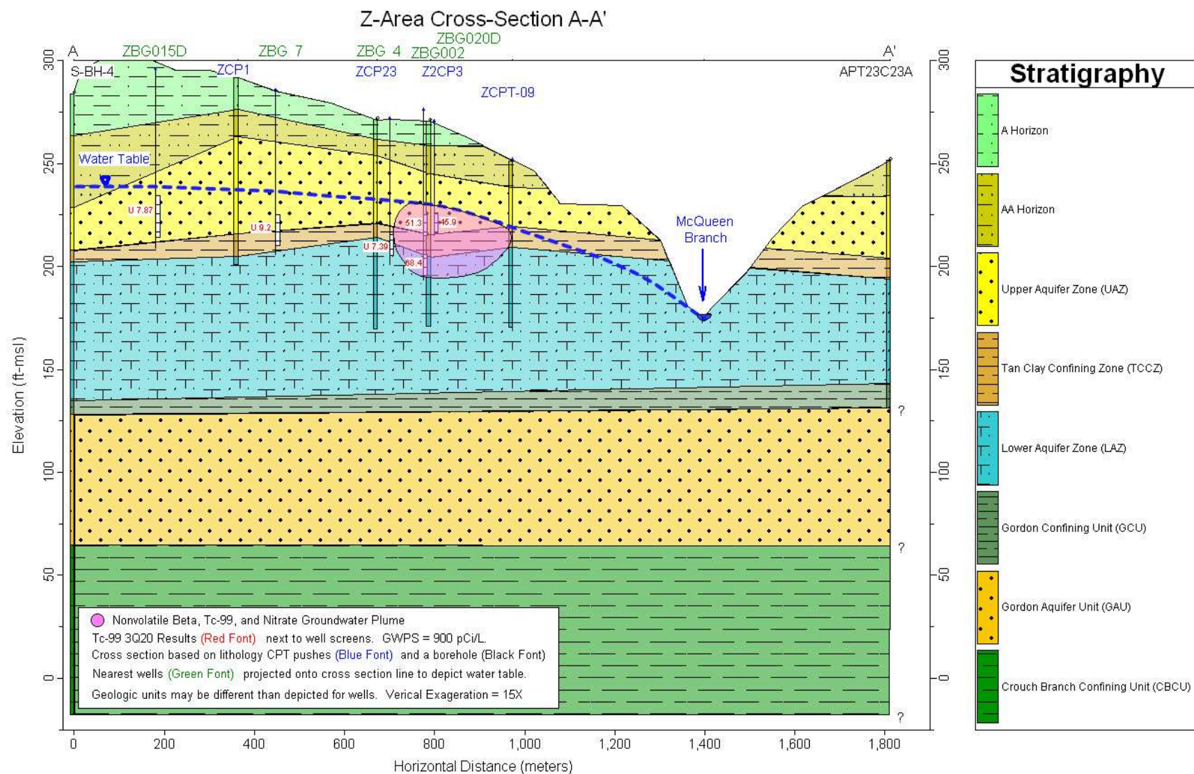
Figure 8. Z-Area Cross Section with 3Q20 Water Table
