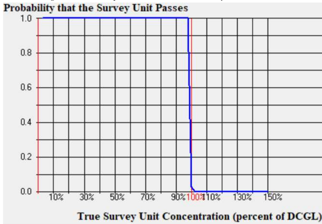
Figure 16-4 - Retrospective Power Curve for Survey Unit B3-012-104
