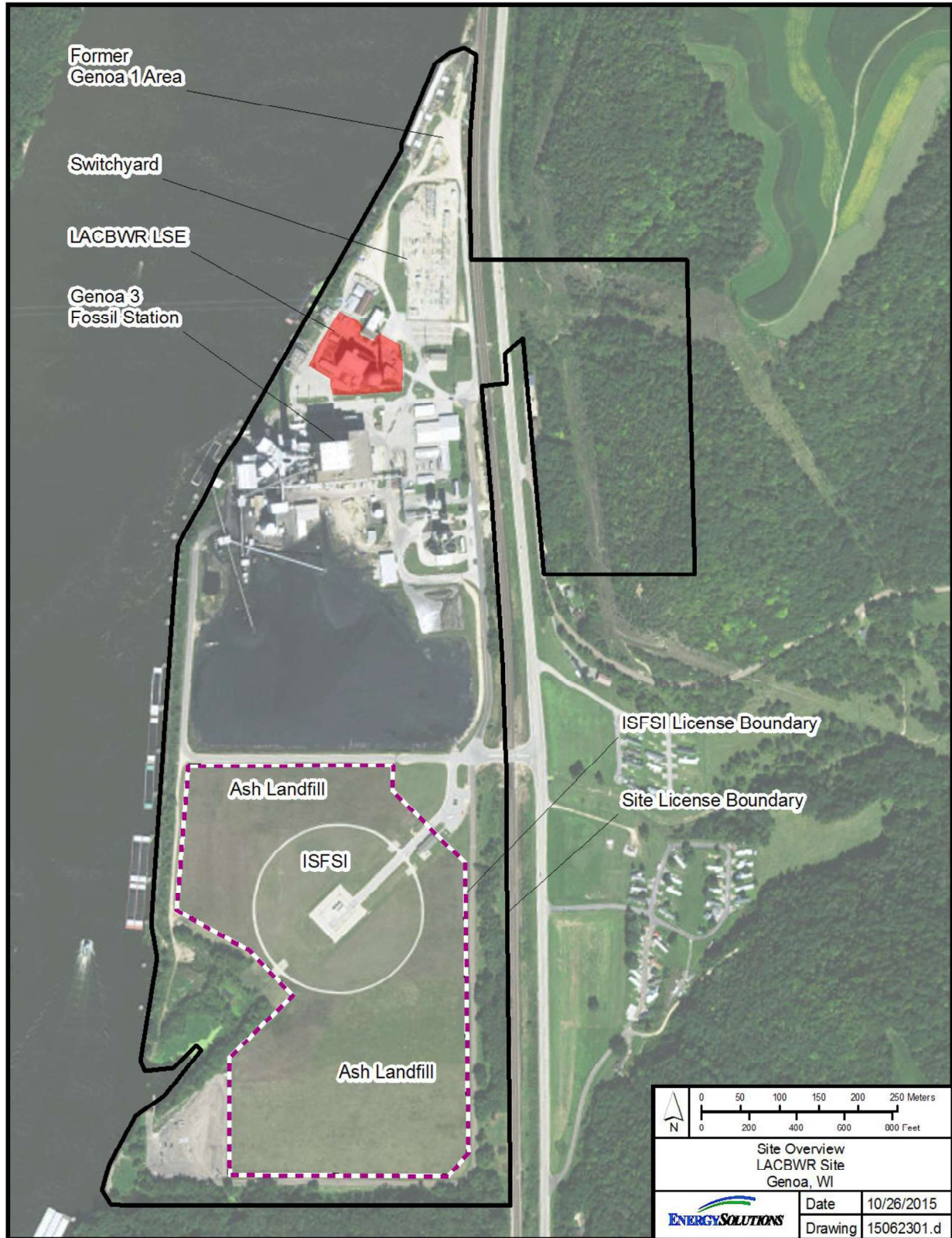
Figure 3-2 Site Overview
