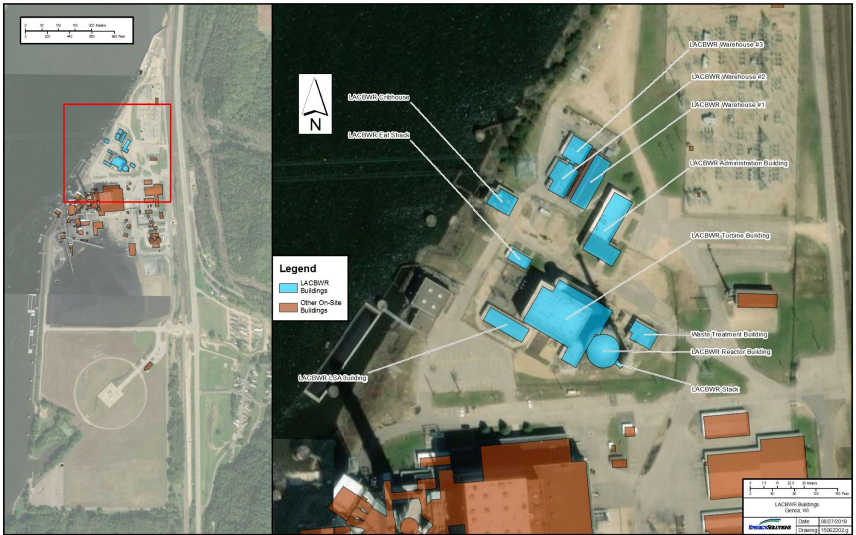
Figure 3-3 LACBWR Buildings
