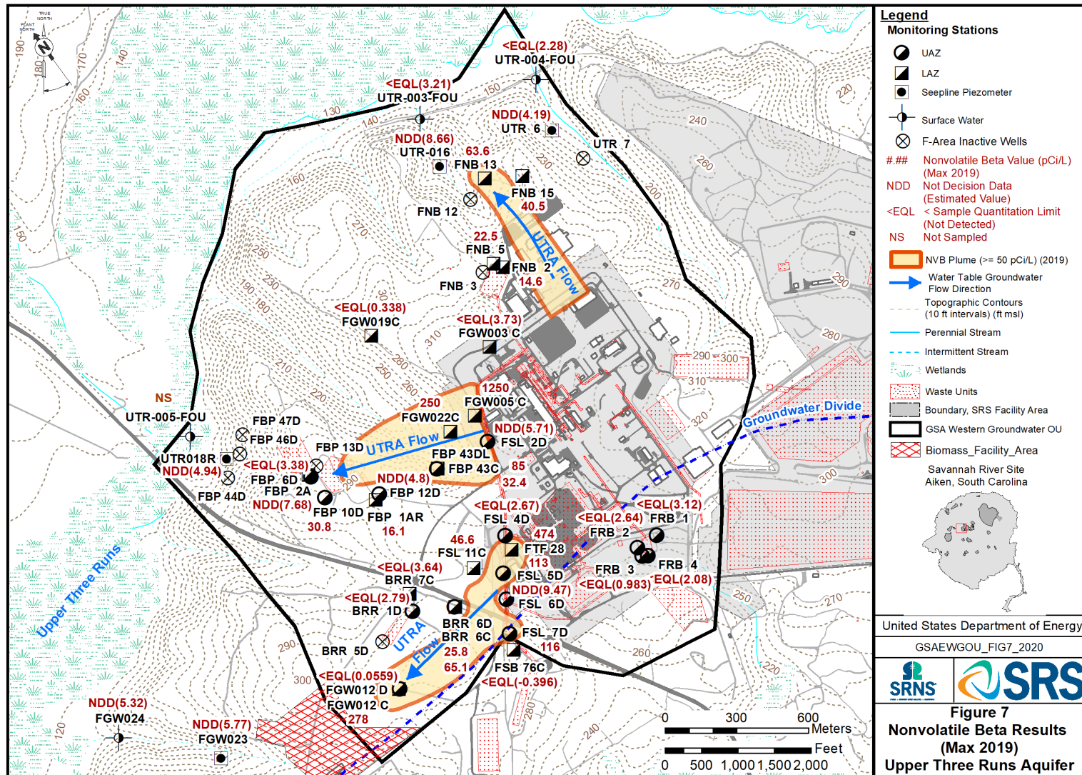
Figure 7. Nonvolatile Beta Results (Max 2019) Upper Three Runs Aquifer
