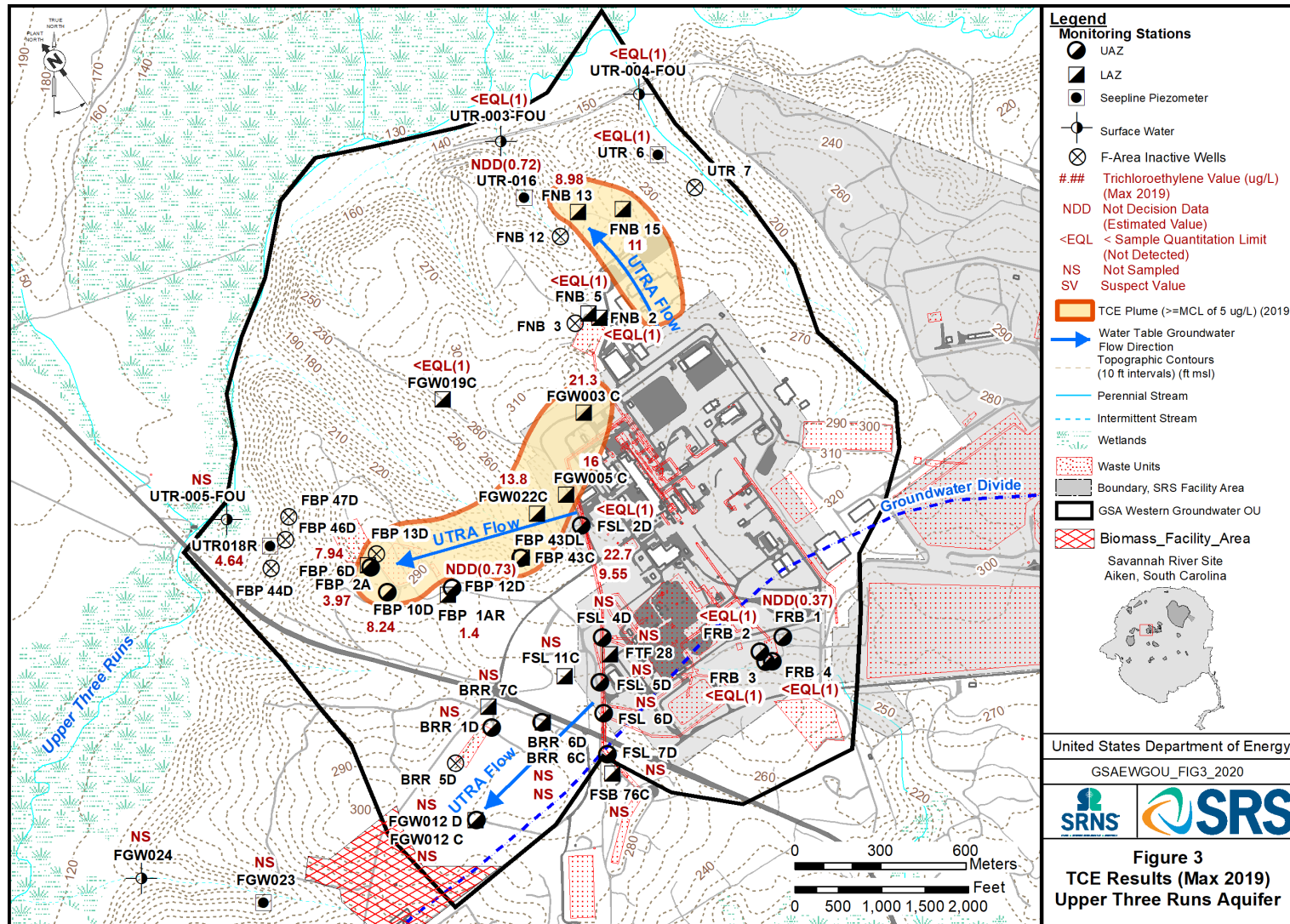
Figure 3. Trichloroethylene Results (Max 2019) Upper Three Runs Aquifer
