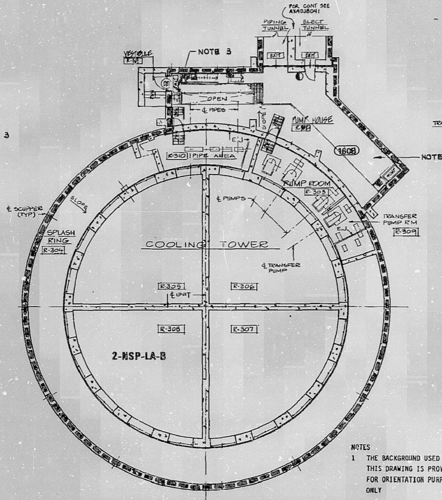
PLAN-GROUND LEVEL - TRAIN "B2"
