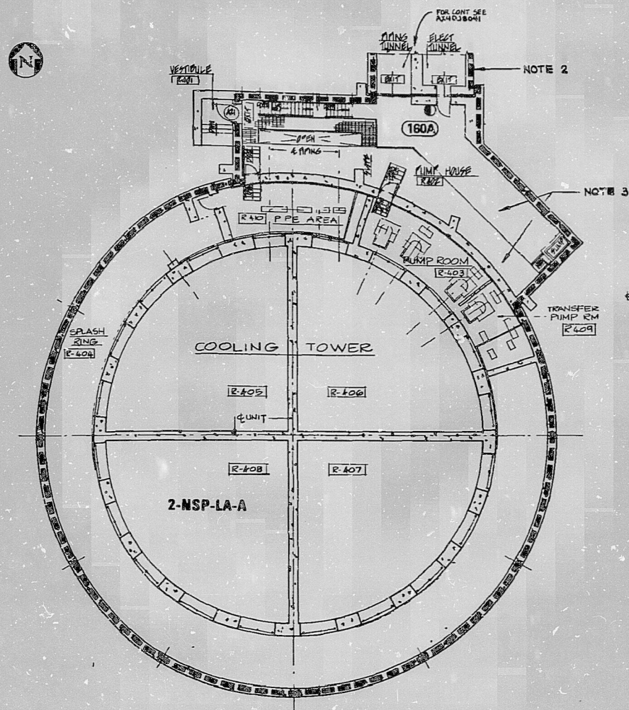
PLAN-GROUND LEVEL - TRAIN "A2"
