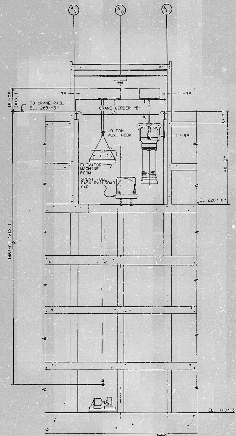
AUXILIARY BLDG.
