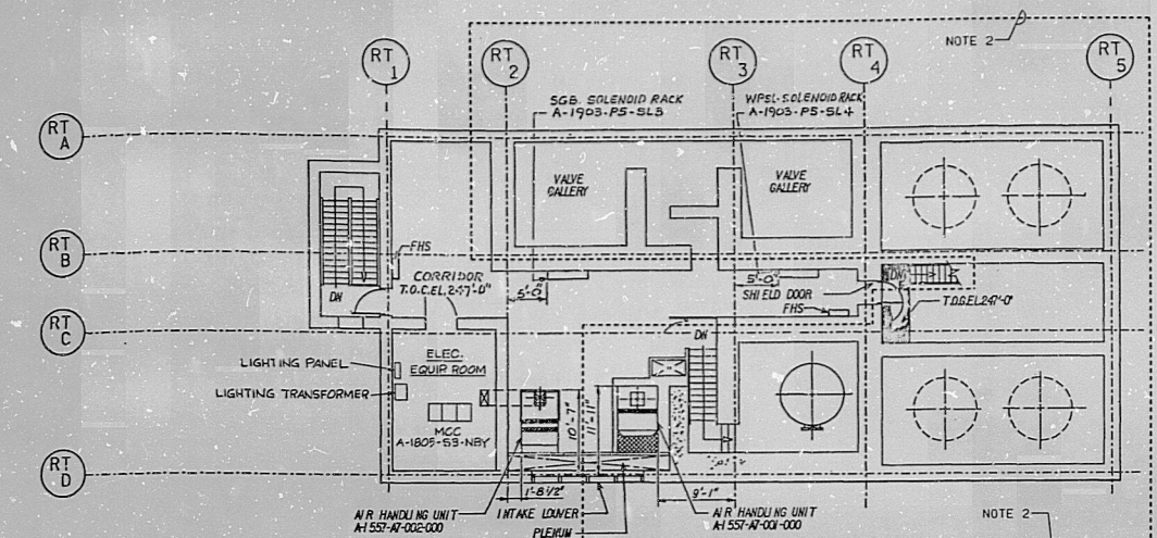
PLAN @ EL.247'-0" & ABOVE
