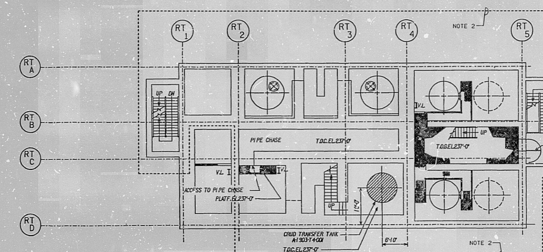
PLAN @ EL.237'-0"
