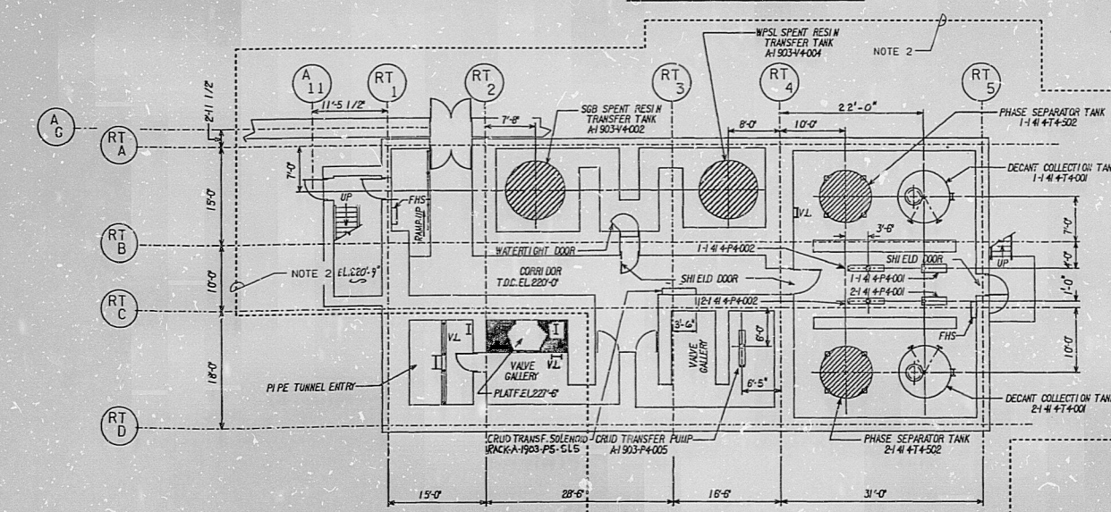
PLAN @ EL.220'-0"
