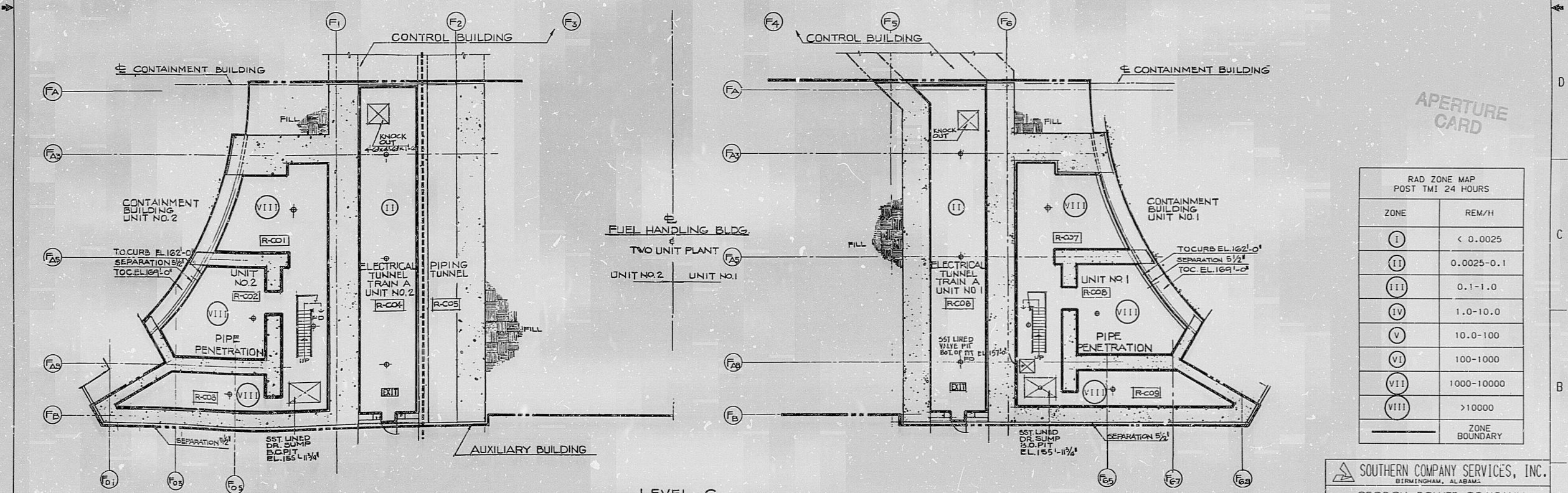
LEVEL C FLOOR PLAN EL.160'-0"
