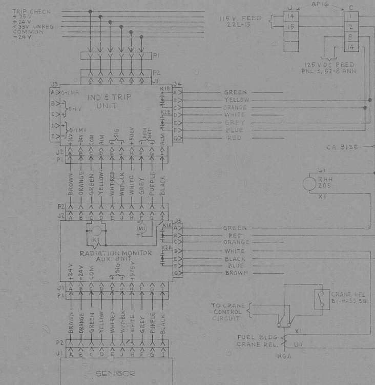
WIRING DIAGRAM FUEL BLDG RADIATION MONITOR
