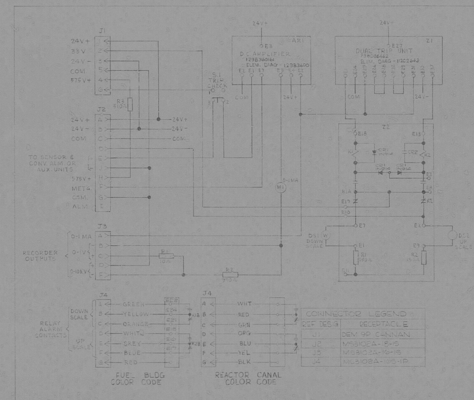
WIRING DIAGRAM INTERNAL CONNECTIONS OF RADIATION MONITOR AND CRANE & TRIP UNIT
