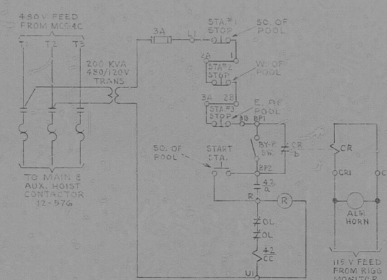
SCHEMATIC DIAGRAM CONTROL FOR FUEL BLDG CRANE
