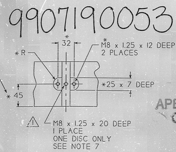
DETAIL B SCALE: 1/2 TYPICAL 4 PLACES
