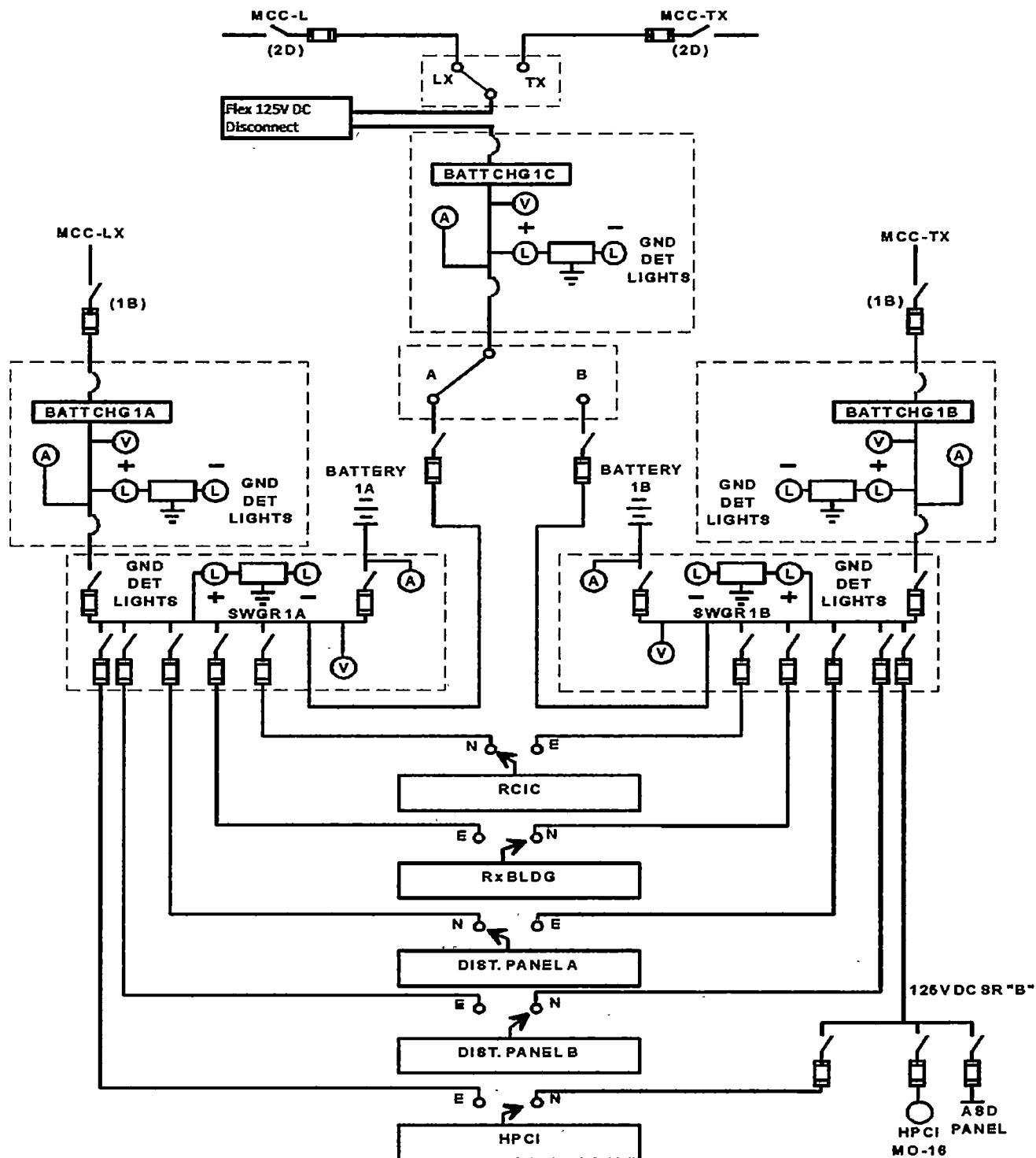
Figure S-2: 125 VDC Power System
