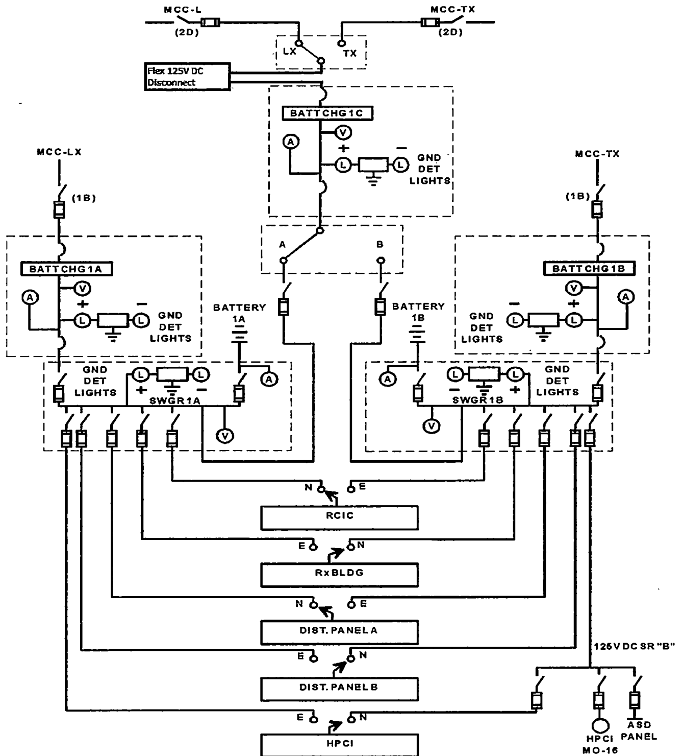
Figure C-2: 125 VDC Power System
