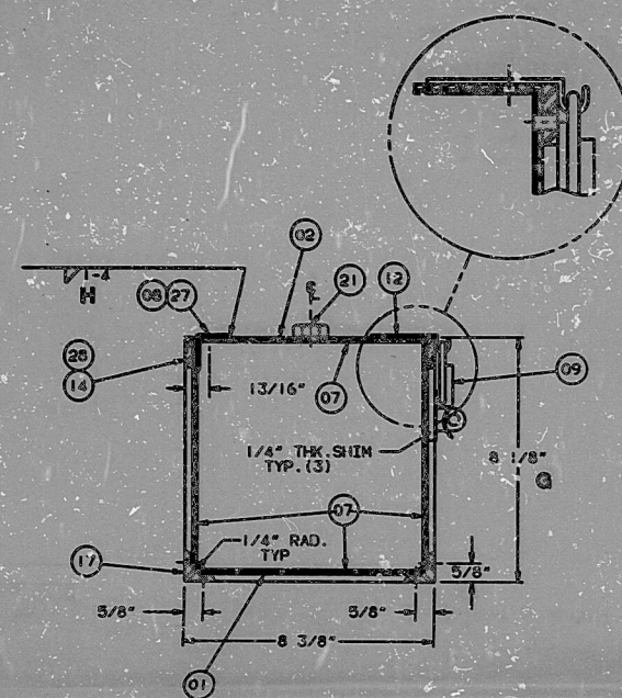
SECTION D-D FROM SHT. 01
