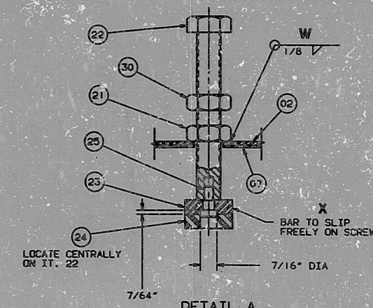
DETAIL A TYPICAL FROM SHT. 01
