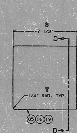
SECTION C-C FROM SHT. 01 SHELL NOT SHOWN
