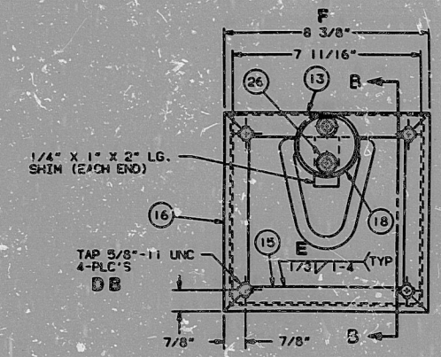
VIEW A-A FROM SHT. 01 SET SCREWS ITEM 10 NOT SHOWN
