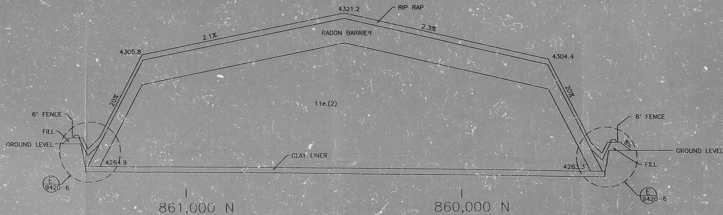
(B) CROSS SECTION 9420-5 HORIZONTAL SCALE: 1" = 100' VERTICAL SCALE 1" = 10'
