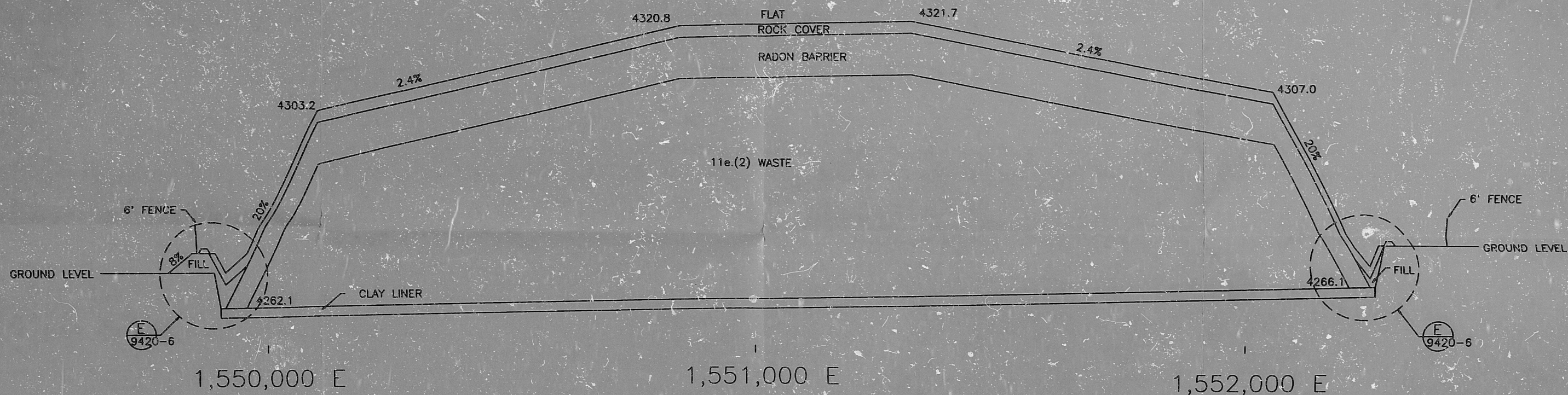
(A) CROSS SECTION 9420-5 HORIZONTAL SCALE: 1" = 100' VERTICAL SCALE 1" = 10'
