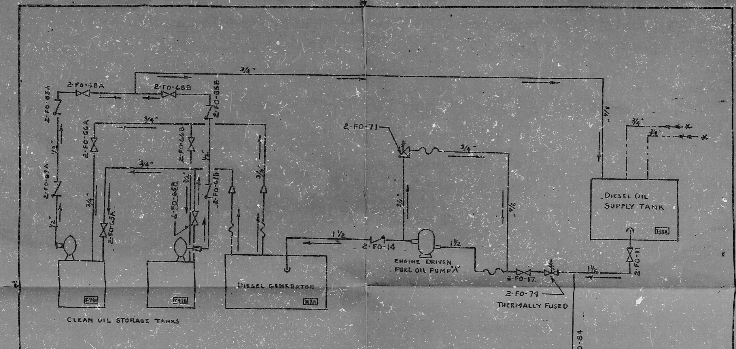
PIPING INSTRUMENT DIAG 25203-26010
