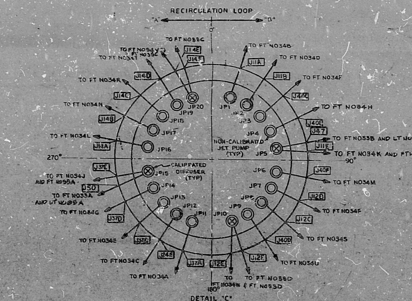
DETAIL 'C' JET PUMP & TRANSMITTER MATCHING DIAGRAM (FOR RELATED EXCESS FLOW CHECK VALVES AND CONTAINMENT PENETRATION ARRANGEMENT SEE DETAIL A AND CROSS REFERENCE TABLE ON SHEET 1)
