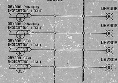
REMOTE CONTROL PANEL OOC381
