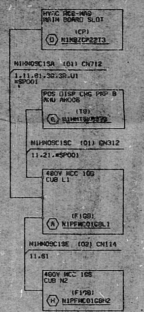
CABLE BLOCK DIAGRAM 1 SCHEME N1HMA09C1 M.A.B. HVAC PDS DISPL CHG PUMP CUB COOLER AHU (N1HMAH006)
