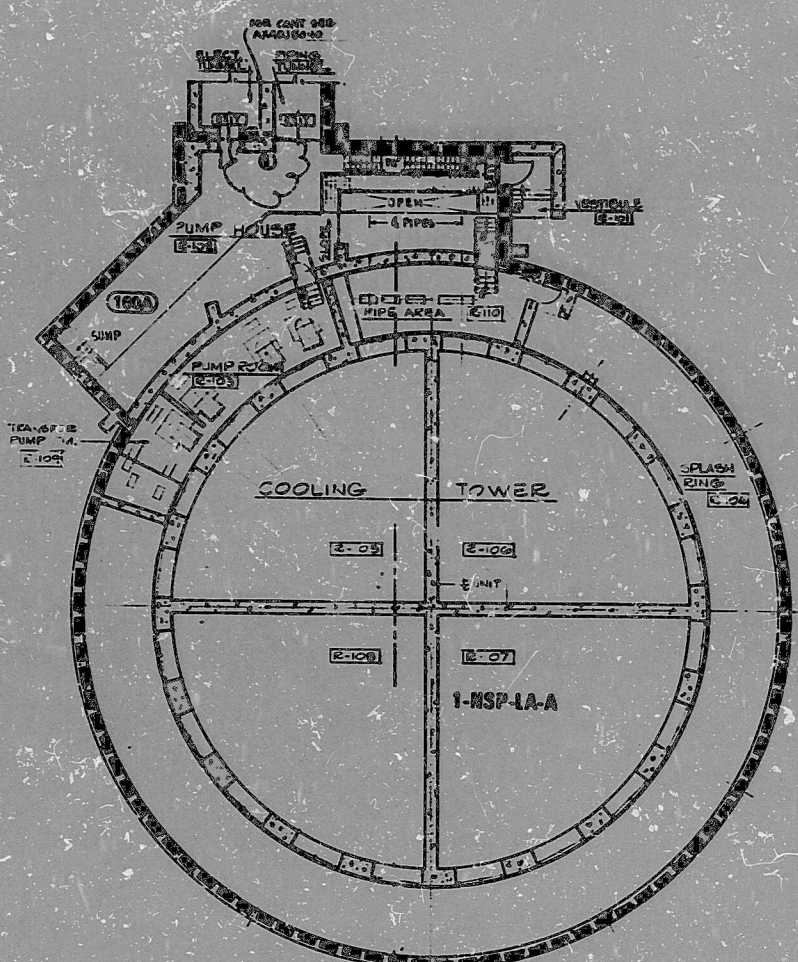
PLAN - GROUND LEVEL - TRAIN "A"
