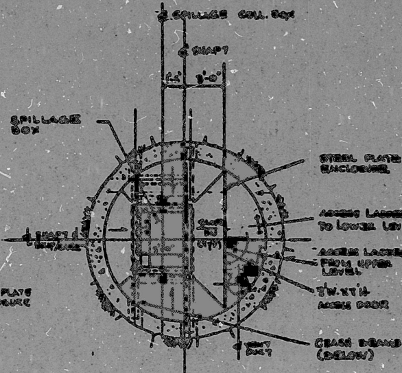
SECTION G-G SCALE: 1/4"=1'-0" FS-GA-014
