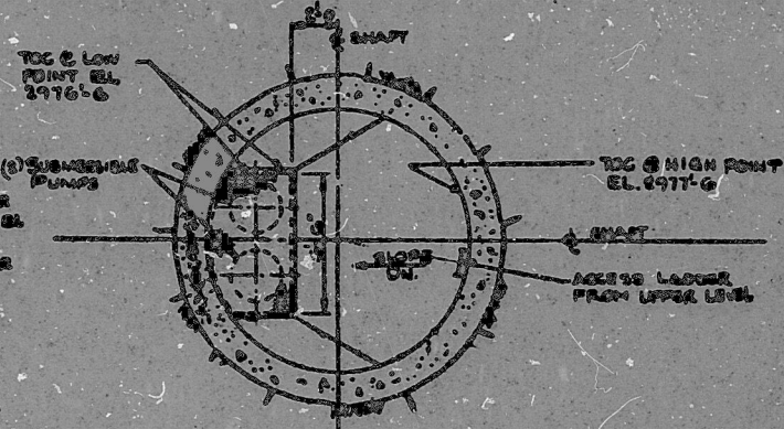
SECTION H-H SCALE: 1/4"=1'-0" FS-GA-015
