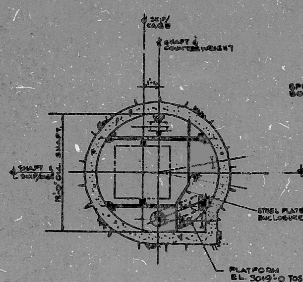
SECTION F-F SCALE: 1/4"=1'-0" FS-GA-013
