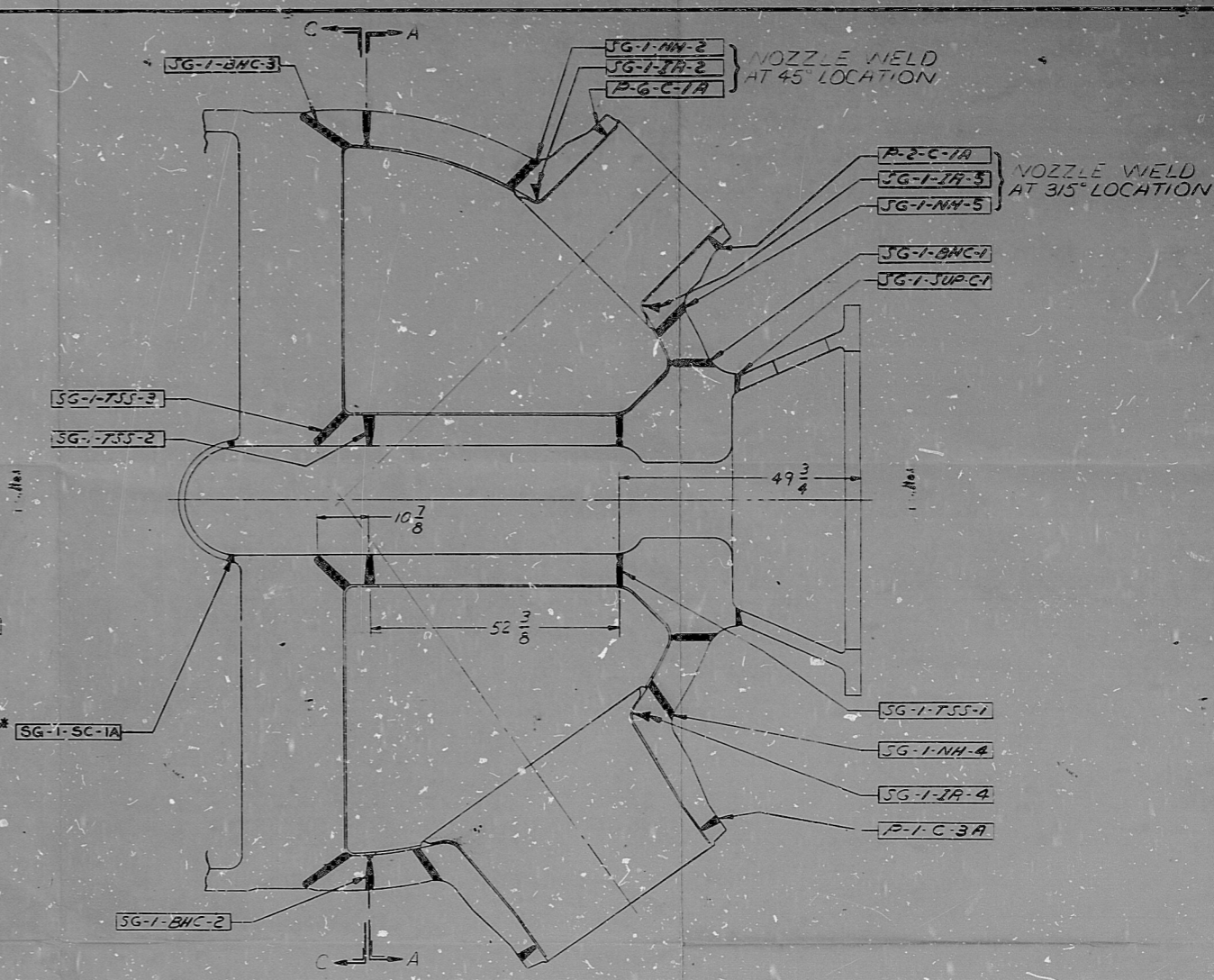
SECTIONAL ELEVATION SCALE: 1"=1'-0"
