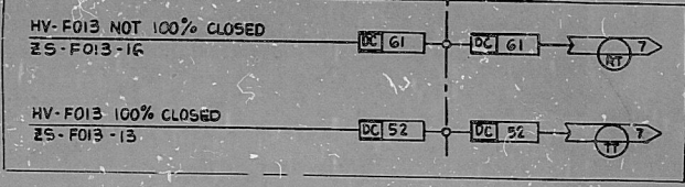
LOGIC FOR HV-FO13 ONLY
