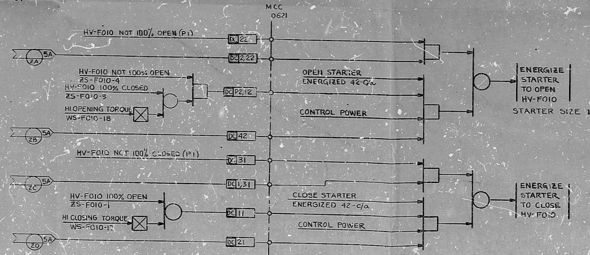
PUMP SECTION FROM CST VALVE HV-FO10 CLASS IE CHANNEL B
