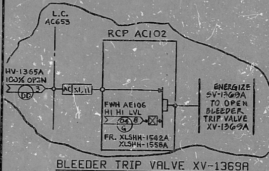
BLEEDER TRIP VALVE XV-1369A
