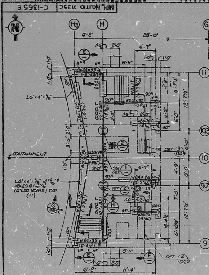
PARTIAL STEEL FRAMING PLAN - RVCU PUMP ROOF EL 125'-0" SCALE 1/8" = 1'-0" SEE DWGS, C-1361, C-1362, C-1365A, C-1366
