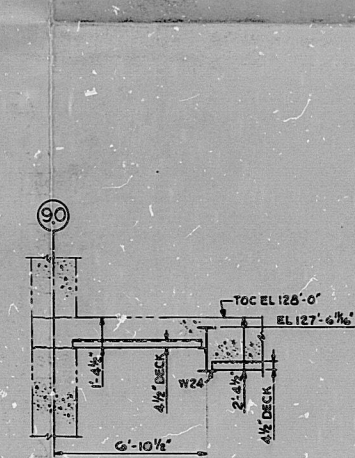
SECTION SCALE 3/8" = 1'-0"
