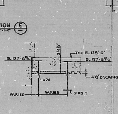
SECTION SCALE 3/8" = 1'-0"
