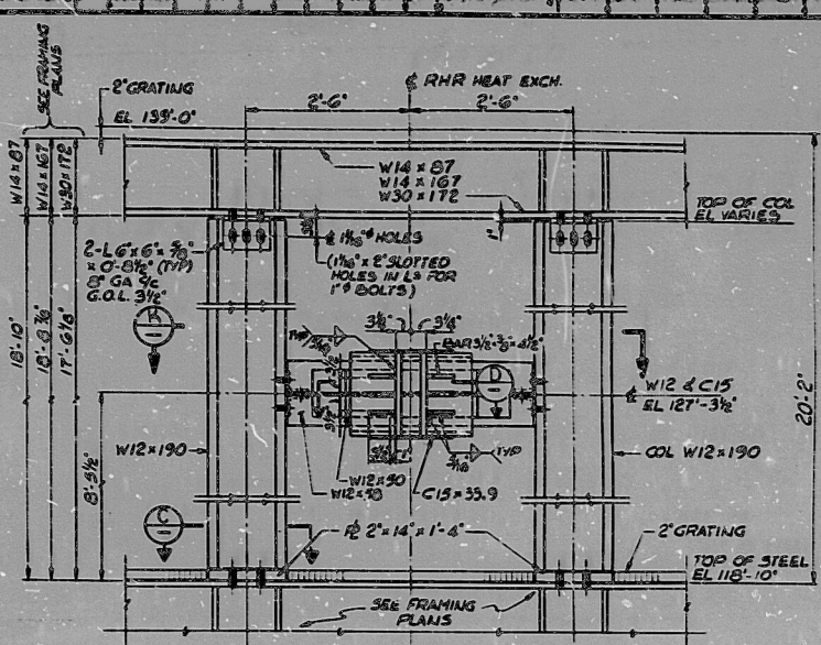
ELEVATION SCALE 1/8" = 1'-0" TYP 4 SIDES SEE DWGS C-1361, C-1362, C-1365, C-1366
