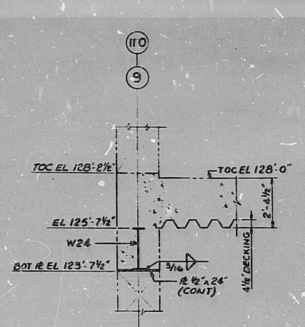
SECTION SCALE 3/8" = 1'-0"
