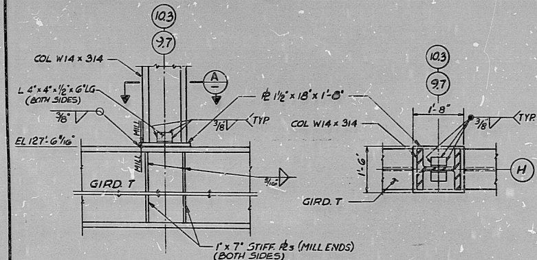
DETAIL SCALE 3/8" = 1'-0"
