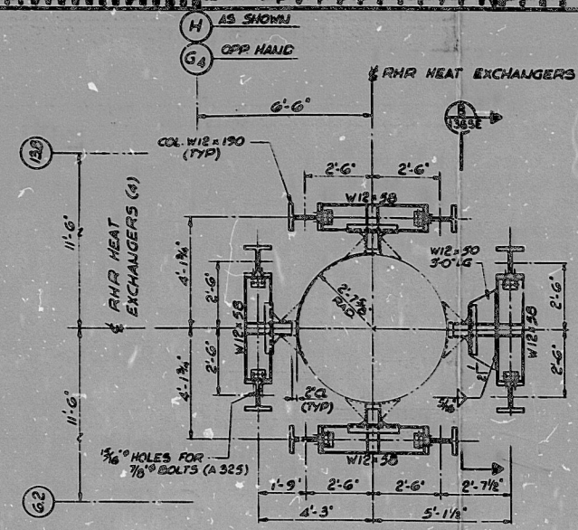
SECTION PLAN SCALE 1/8" = 1'-0" 2 PLACES - AS SHOWN 2 PLACES - OFF HAND SEE DWGS, C-1361, C-1362, C-1365A, C-1366
