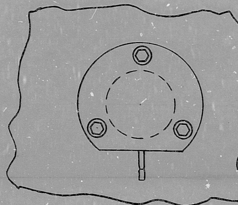
BOTTOM VIEW OF SECTION "A-A" SHOWING ORIENTATION OF SG SOURCE CAPSULE
