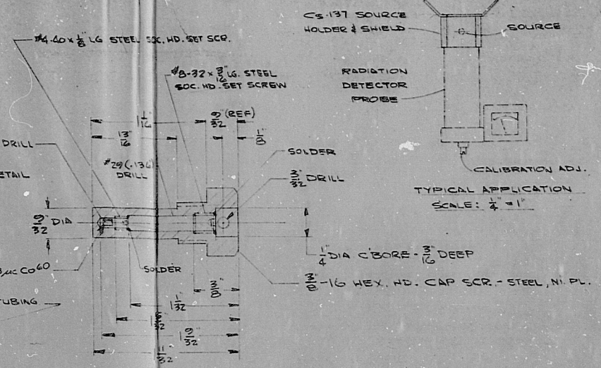
CO-60 SOURCE HOLDER DETAIL SCALE: 2" = 1"
