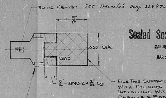
CS-137 SOURCE CONTAINER & PLUG SCALE: 2" = 1"
