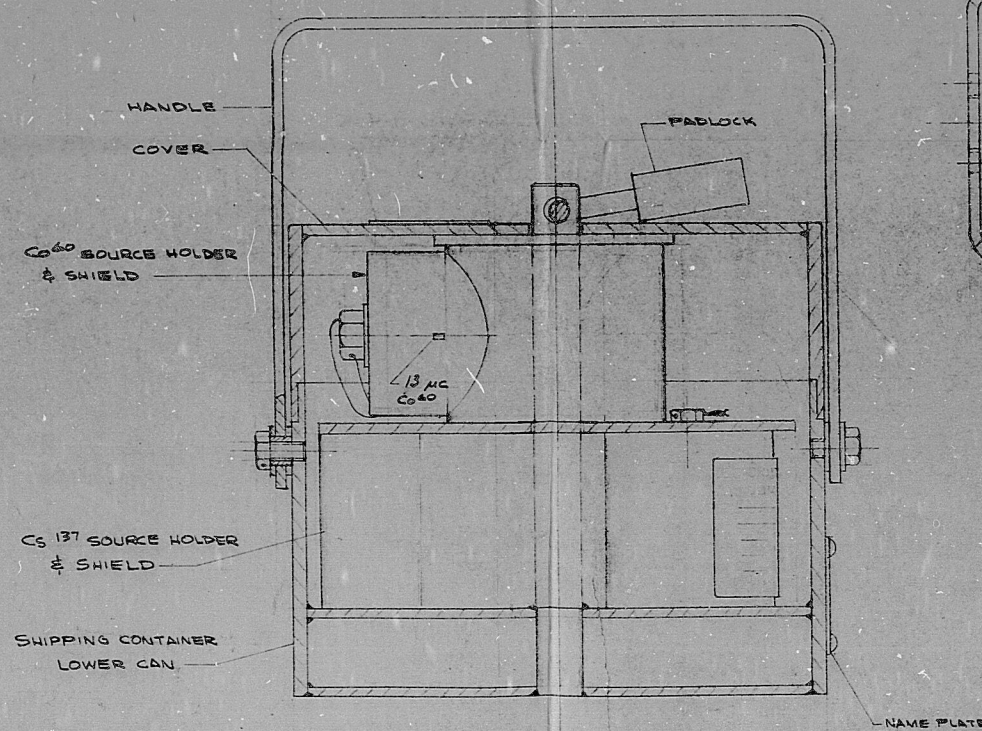
SHIPPING CONTAINER WITH SOURCE HOLDER & SHIELD
