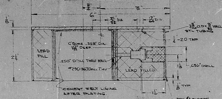
PLAN VIEW - SOURCE SHIELD NOT SHOWN.
