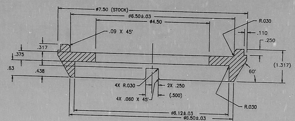
SECTION C-C SCALE 1/1
