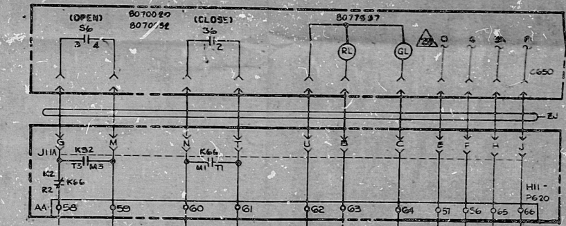
PUMP DISCHARGE VALVE E41-F007 (DC) SEE FIG 14 REF 19
