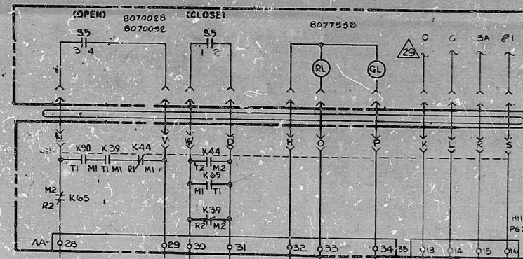
PUMP DISCHARGE VALVE CS E41-F006 (DC) SEE FIG 14 REF 19
