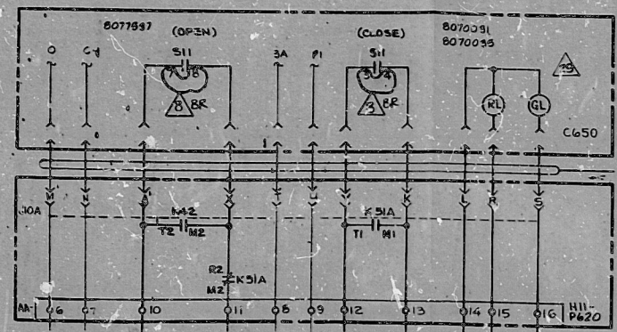
PUMP SUCTION FROM SUPPRESSION CHAMBER VALVE E41-F002 (DC) SEE FIG 14 REF 19
