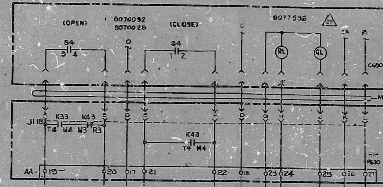
PUMP SUCTION FROM CONDENSATE STORAGE TANK VALVE E41-F004 (DC) SEE FIG 14 REF 19
