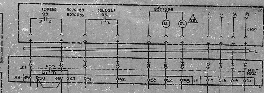
STEAM SUPPLY TO TURBINE VALVE E41-F001 (DC) SEE FIG 13 REF 19
