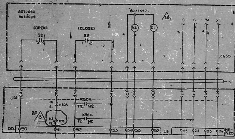
STEAM SUPPLY LINE ISOLATION VALVE E41-F003 (AC) (OUTBOARD) SEE FIG 14 REF 19
