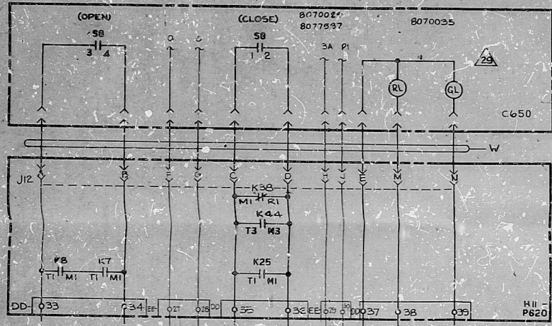
REDUNDANT SHUTOFF TO CONDENSATE STORAGE TANK VALVE E41-F011 (DC) SEE FIG 12 REF 19
