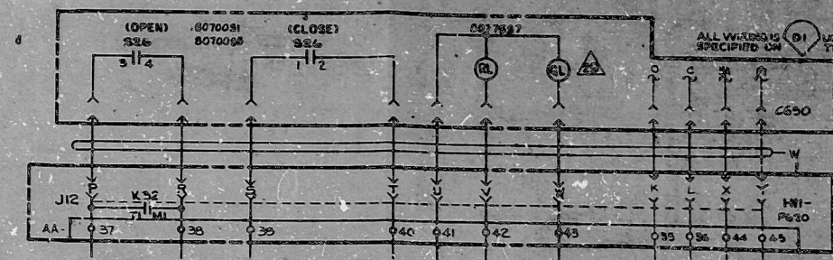
LUBE OIL COOLING WATER VALVE E41-F039 (DC) SEE FIG 13 REF 19
