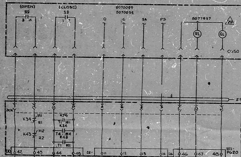
REDUNDANT SHUTOFF TO CONDENSATE STORAGE TANK VALVE E41-F011 (DC) SEE FIG 12 REF 19
