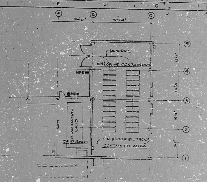
FLOOR PLAN ELEV. 796'-0" CHLORINATION BUILDING FOR CIRCULATING WATER INTAKE STRUCTURE SCALE: 1/8" = 1'-0"
