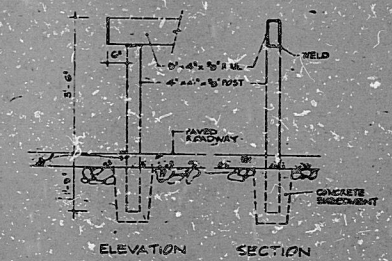
ELEVATION SECTION DETAIL VEHICLE GUARD RAIL SCALE: 1/4" = 1'-0"
